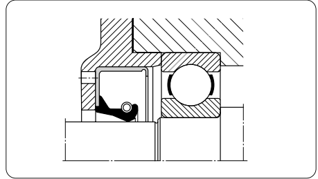
Fig 4. CRW1 seal
