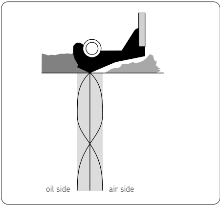
Fig 41. SKF Waveseal lip with sinusoidal edge
