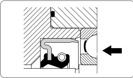
Fig 19. CRWA5 seal
