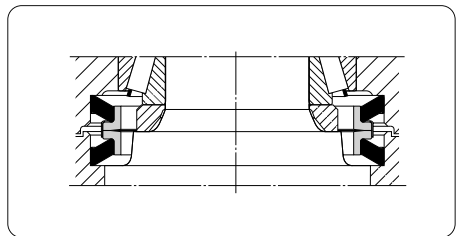
Fig 32. HDDF mechanical seal
