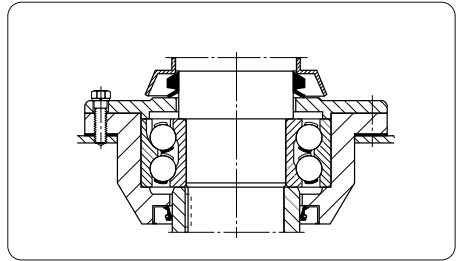
Fig 31. V-ring seal
