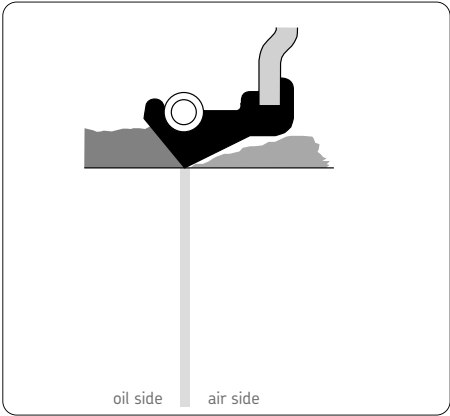
Fig 40. Conventional sealing lip with straight edge
