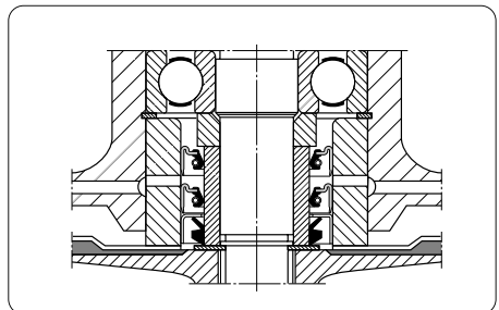
Fig 33. CRW5 seals + V-ring seal
