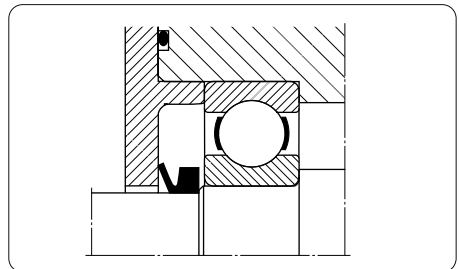
Fig 7. V-ring seal
