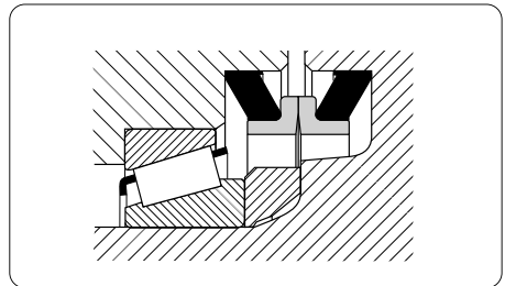
Fig 6. HDDF mechanical seal
