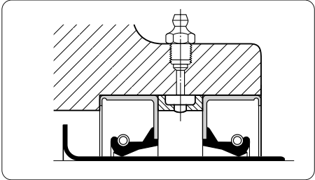
Fig 61. Spacing ring
