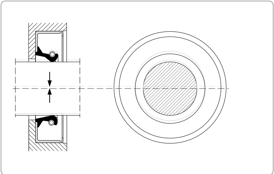
Fig 42. Coaxiality
