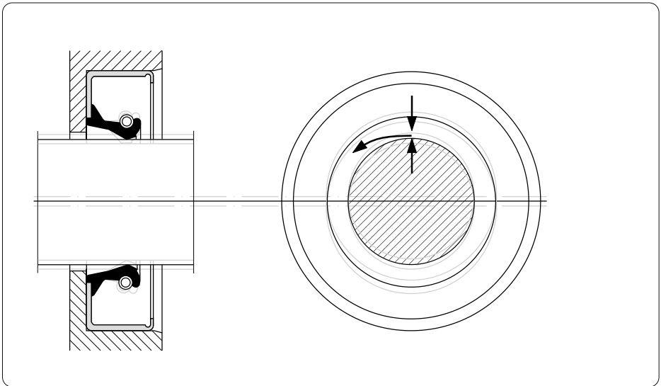
Fig 43. Runout
