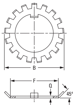
Fig. 50. Lockwashers.
