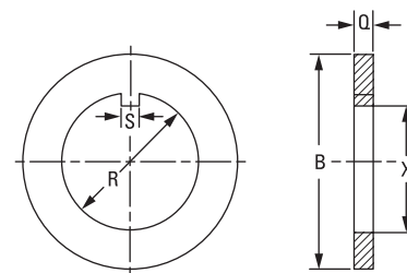
Fig. 51. Tongued washers.
