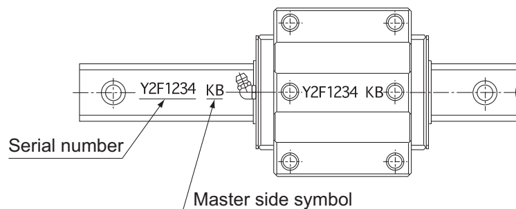
Fig.17 Master LM Rail
