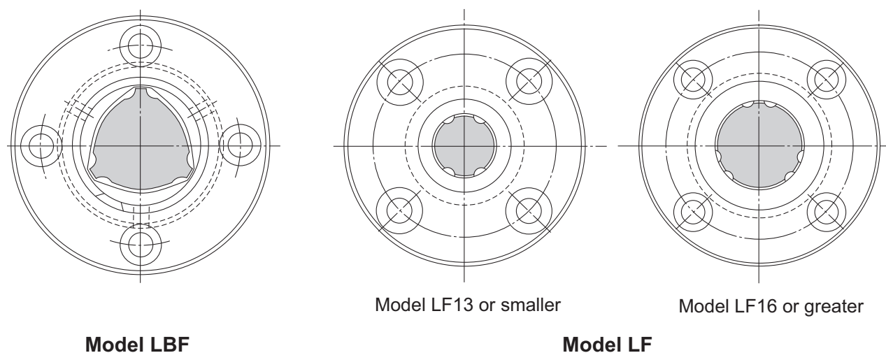
Fig.2 Positions of Flange Mounting Holes
