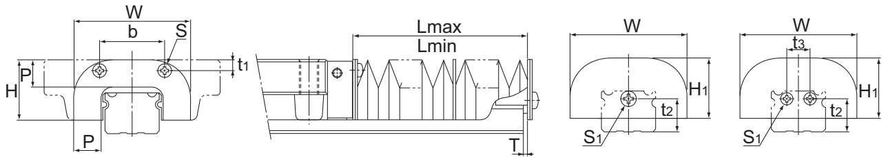
Models SNR25 to 45
