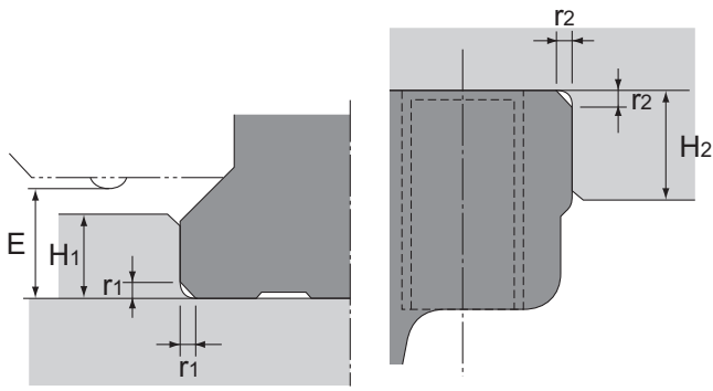
Shoulder for the LM Rail
