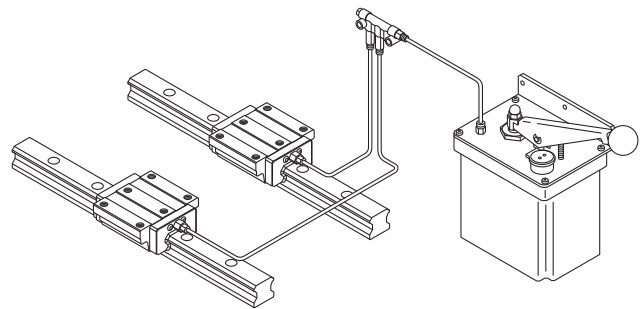
Fig.2 Lubrication through a Centralized Piping System
