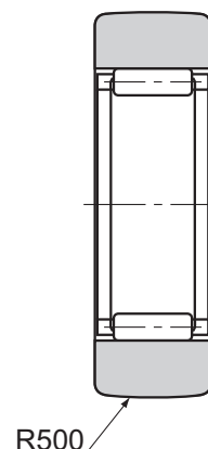
Model RNAS-R
