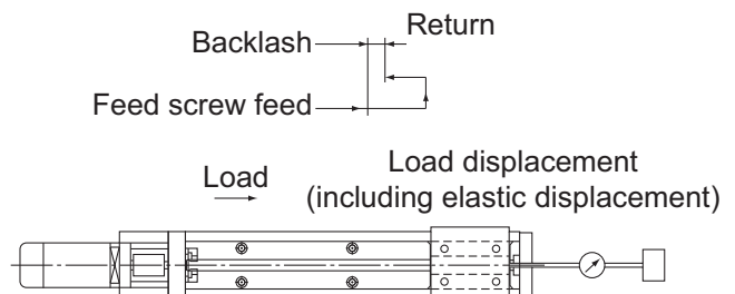
Fig.11 Backlash
