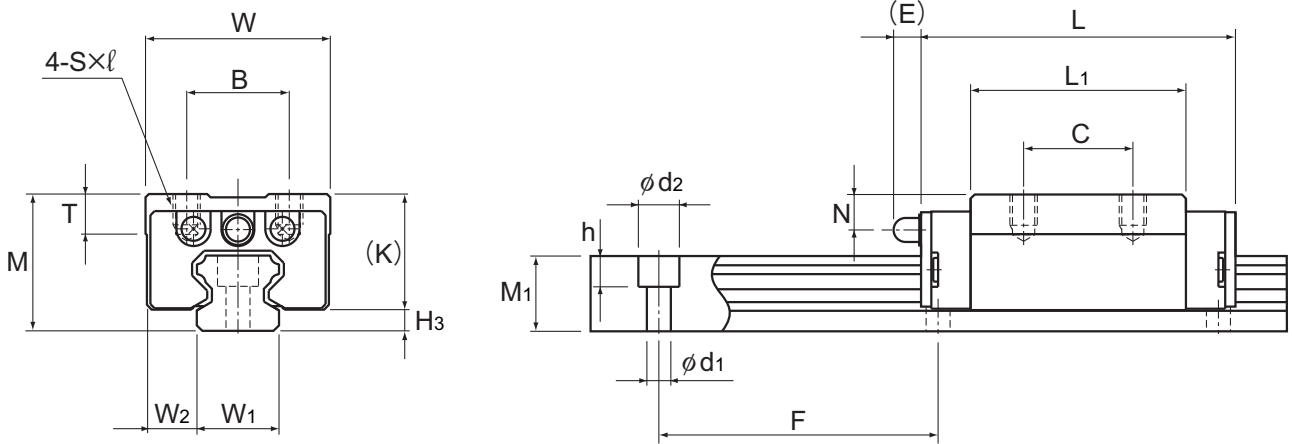
Model HSR12RM
