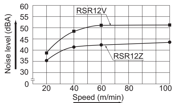
Fig.1 Noise Levels of Models RSR12Z and RSR12V
