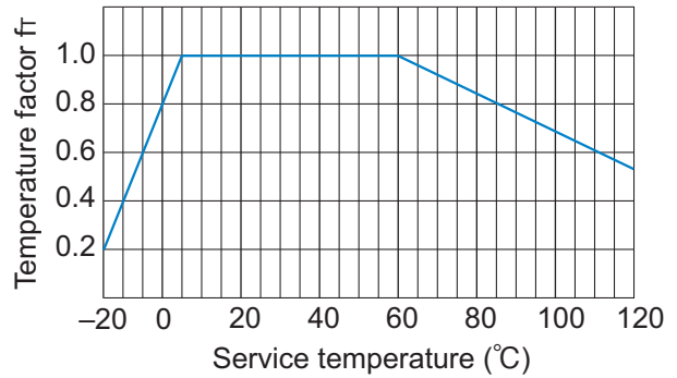
Fig.2 Temperature Factor
