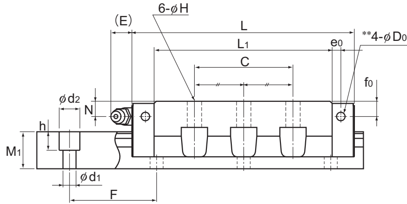
Model NRS-LB
