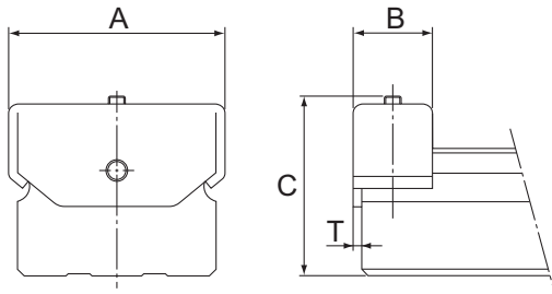
Fig.5 End Piece EP for Models NR/NRS
