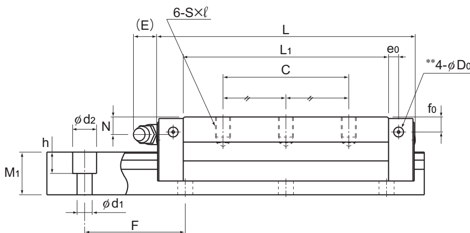
Model SNS-LR
