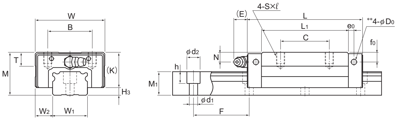
Model NR-R
