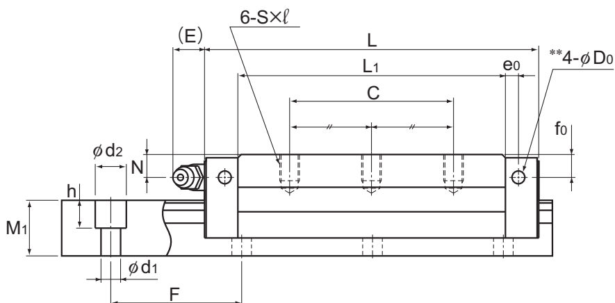
Model NRS-LR
