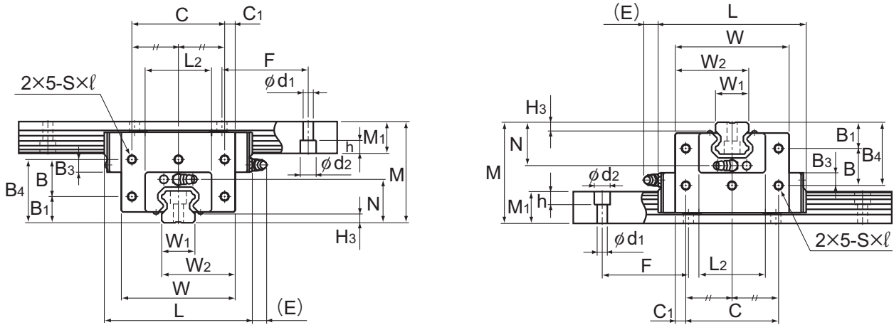
Models CSR20 to 45
