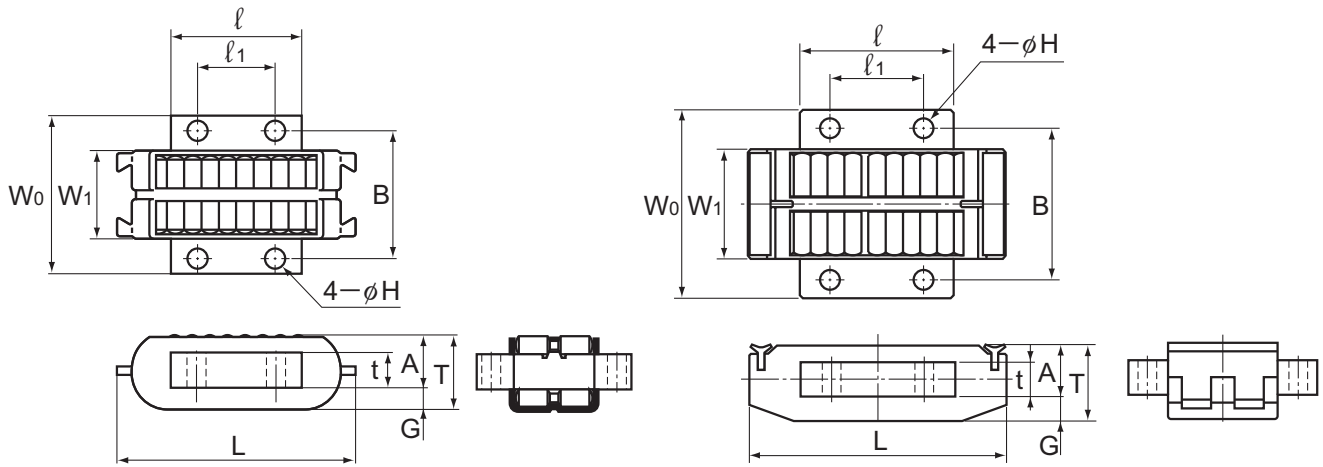
Model LR
