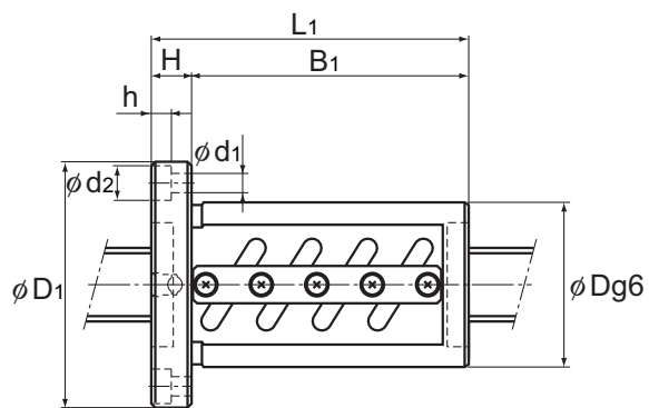
Model BIF
