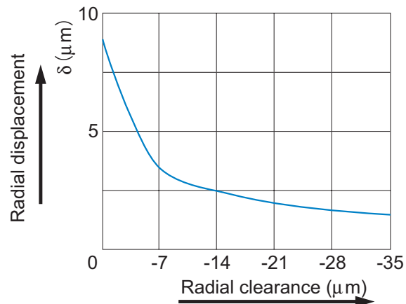
Fig.6 Radial Clearance and Deflection
