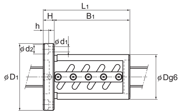
Model BIF
