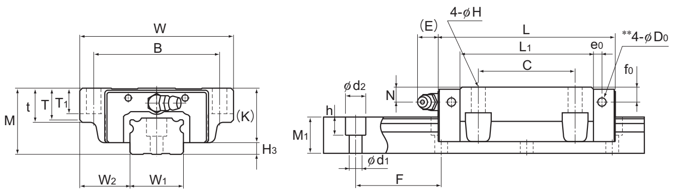
Model NRS-B
