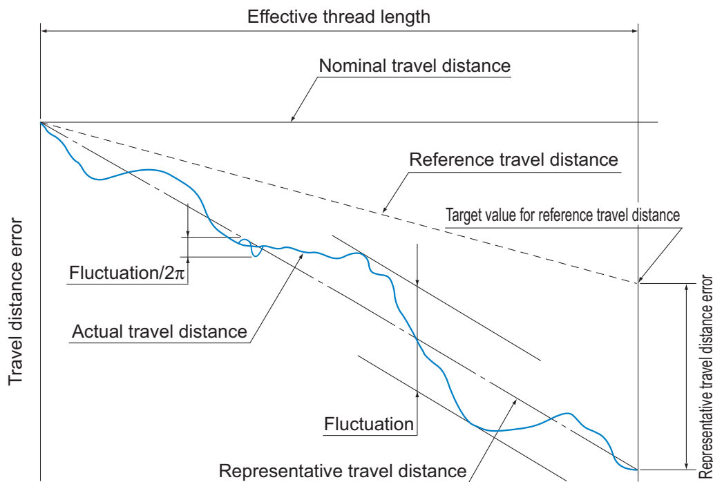
Fig.1 Terms on Lead Angle Accuracy
