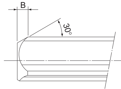
Fig.2 Chamfer B
