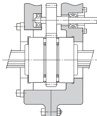
Fig.2 Examples of Fitting the Spline Nut
