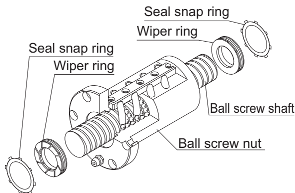
Wiper Ring for the Ball Screw
