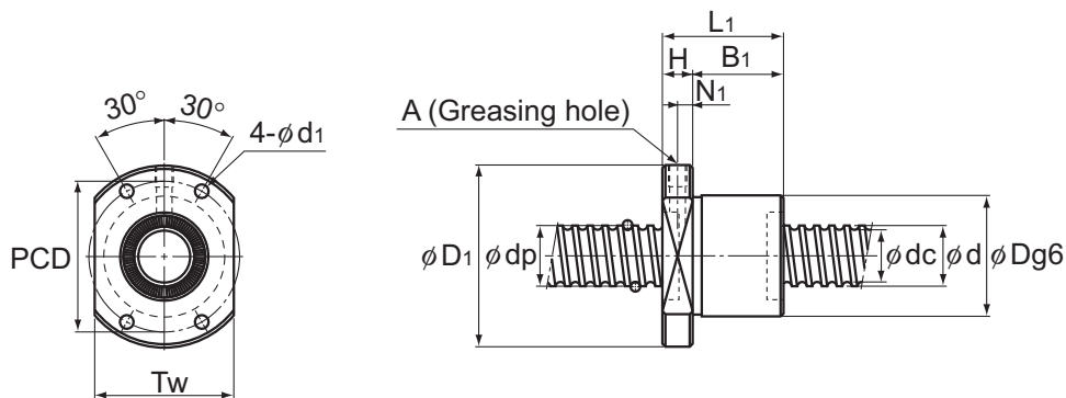
Models BTK 1404 to 5016
