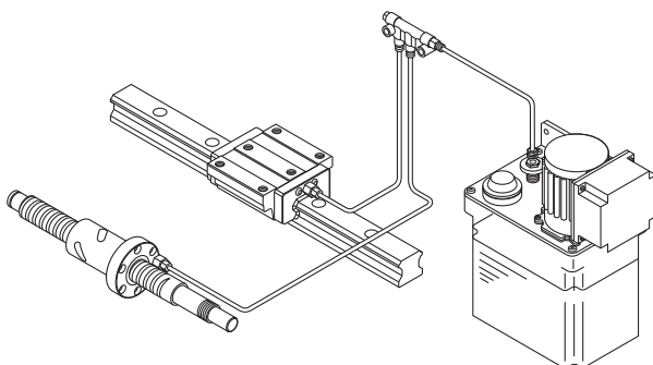
Fig.3 Forced Lubrication Method
