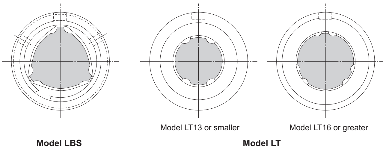
Fig.1 Positions of Keyways
