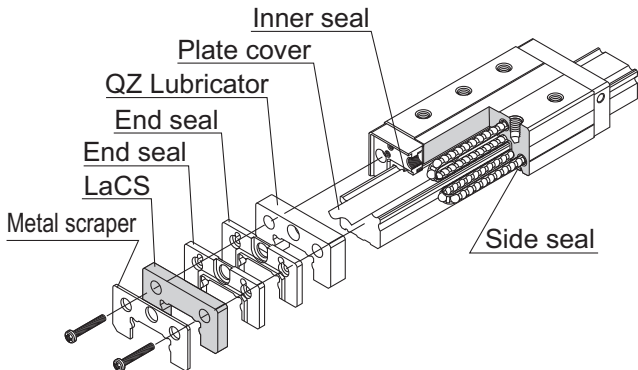
Contamination Protection Seal for the LM Guide
