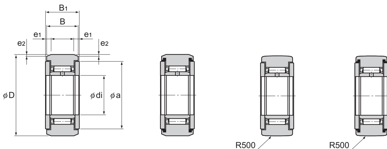
Model NAST-ZZ
