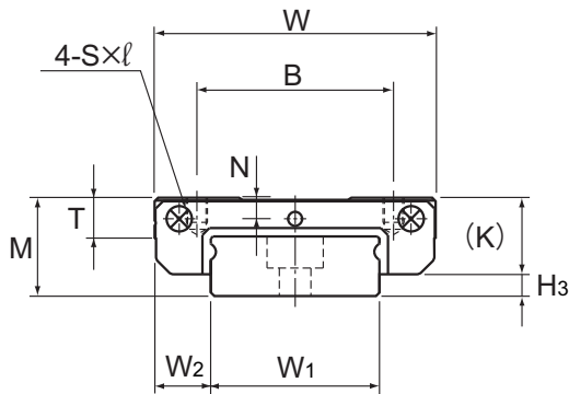
Models SRS7WM, 9WM and 12WM
