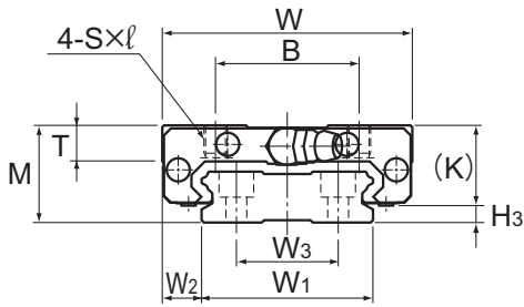
Models HRW17 and 21CR/CRM
