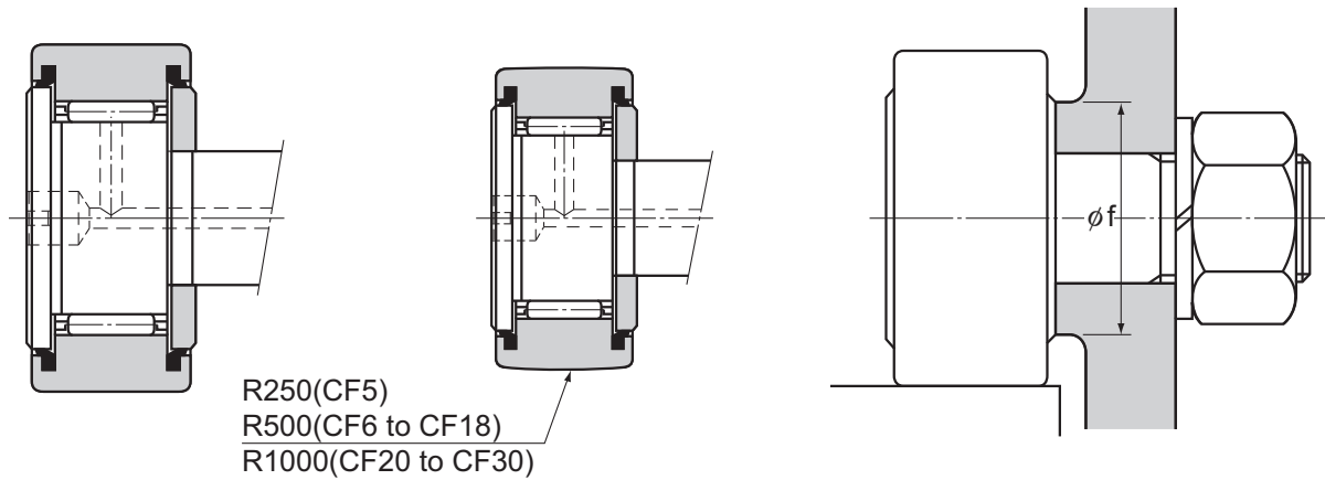
Model CF...UU
