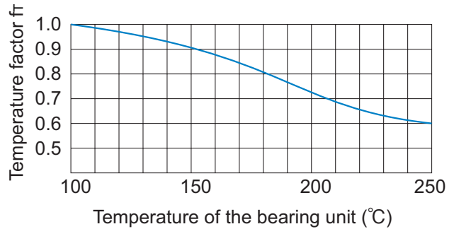
Fig.1 Temperature Factor (f r )
