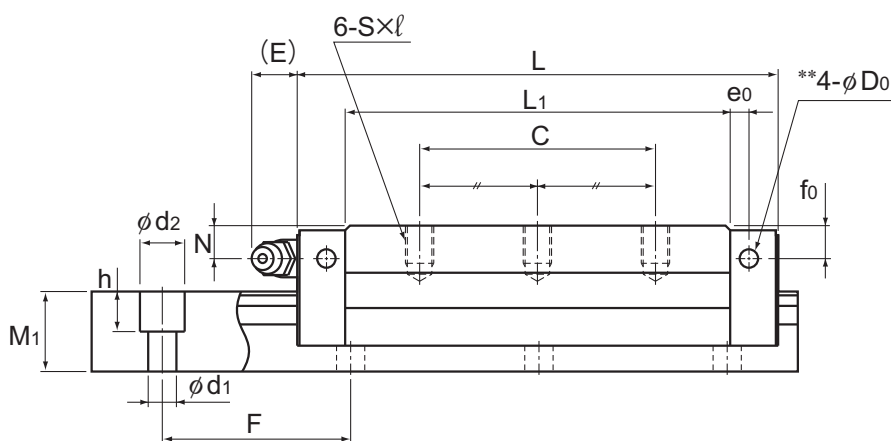
Model NR-LR
