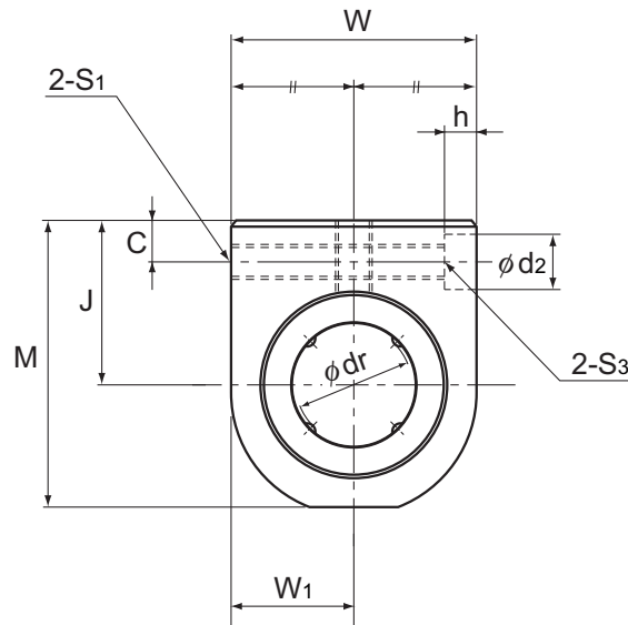
Model SH
