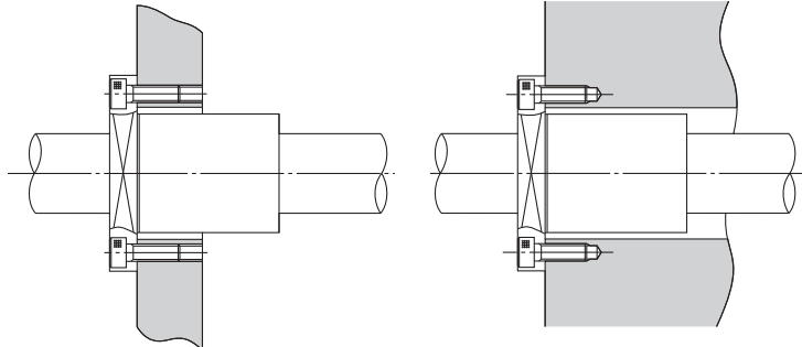
Mounted via a flange only
