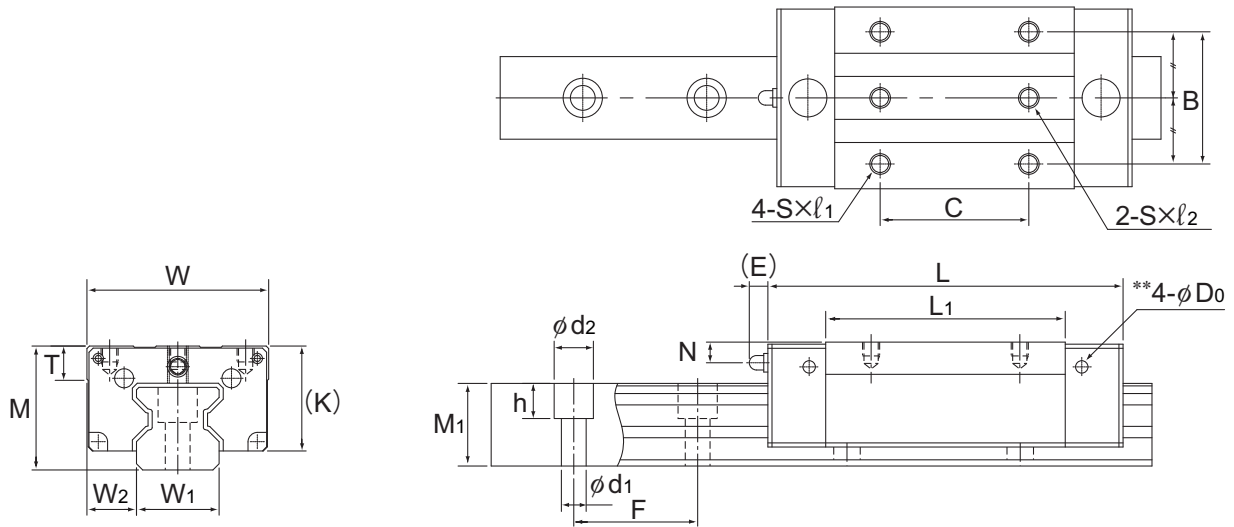
Models SRG15V and 20V/LV
