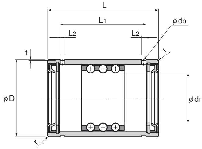
Model ST...UU (For light load)
