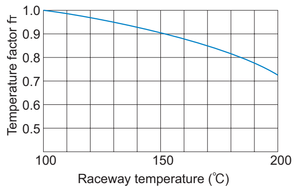
Fig.12 Temperature Factor ( f_T )
