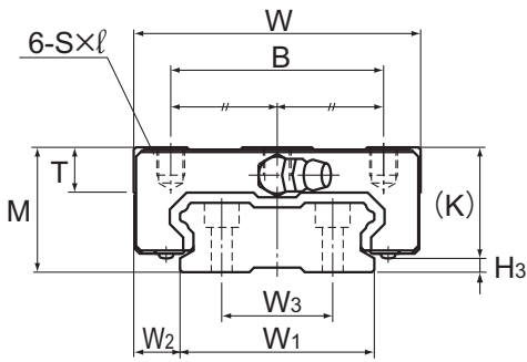
Models HRW27 to 50CR/CRM
