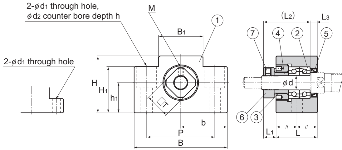
Models EK 4 and 5
