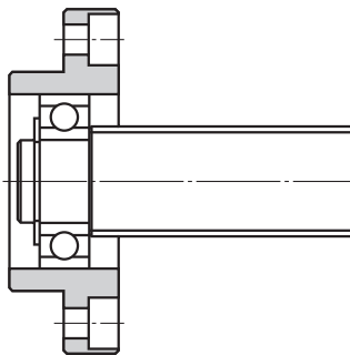
Model FF
