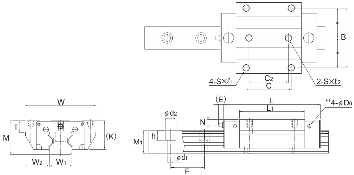
Models SRG15A and 20A/LA
