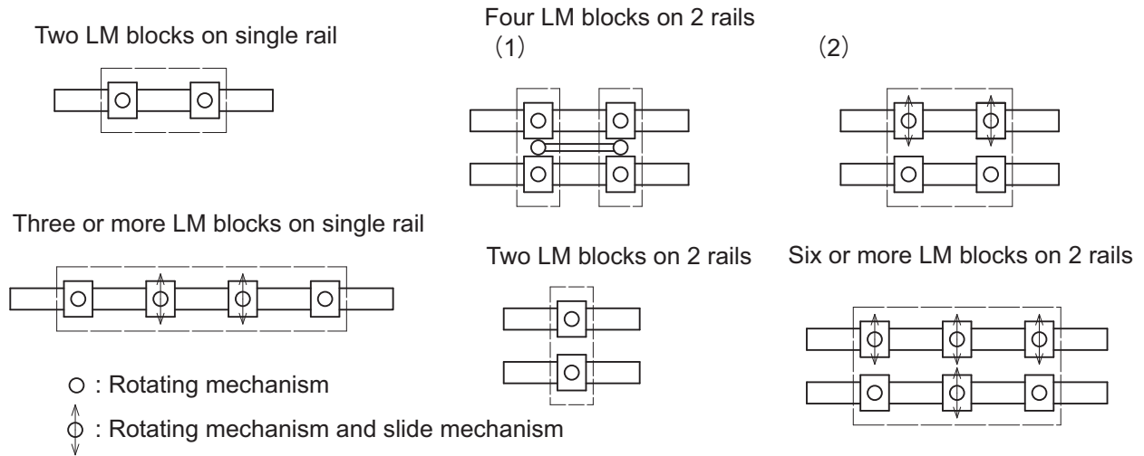
Fig.5 Examples of Table Mechanisms
