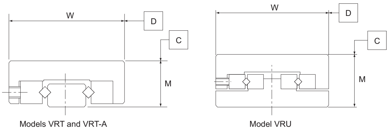
Fig.2 Accuracy Standards
