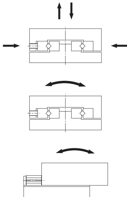
Fig.2 Load Directions
