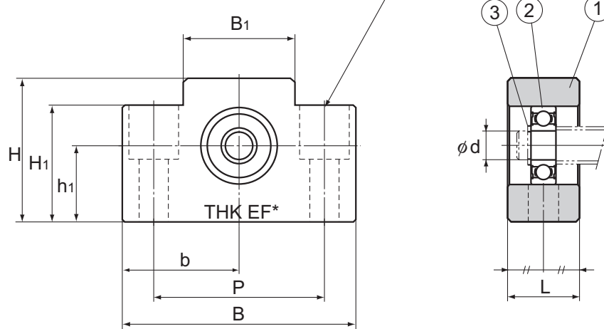
Models EF 6 and 8
