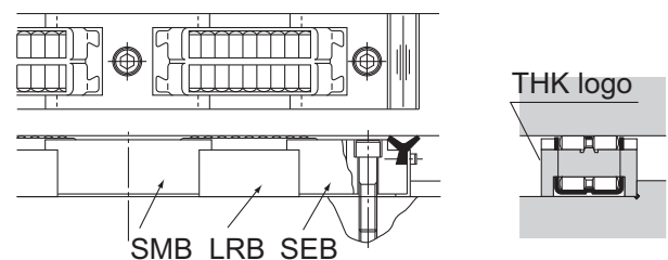
Fig.1 Installing the LM Roller
