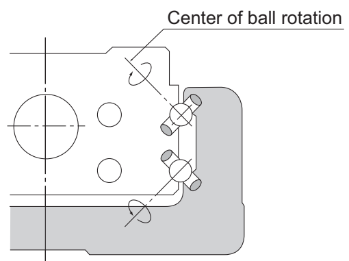
Fig.4 Contact Structure of Model KR
