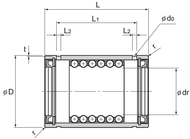
Model ST...UUB (For medium load)
