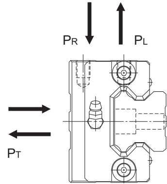
Fig.4 Model HSR-M1YR
