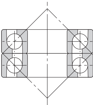
Angular Ball Bearings Mounted Back-to-back (DB type)
