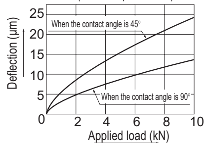
Load and deflection when contact angles are not the same ( D_a=6.35\text{mm} ) (deflection per 24 balls)
