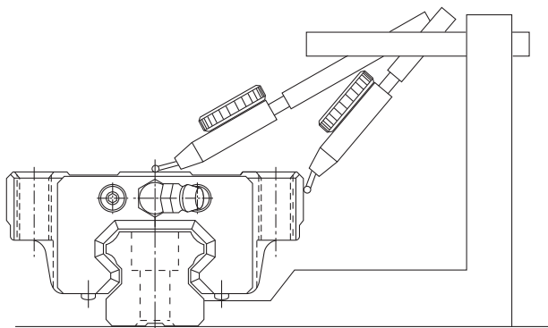
Fig.16 Running of Parallelism
