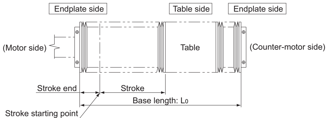
Fig.3 Schematic Drawing of Mounting the Bellows
