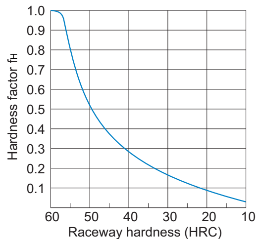
Fig.2 Hardness Factor ( f_H )
