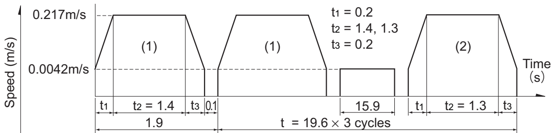
Fig.8 Operating Pattern
