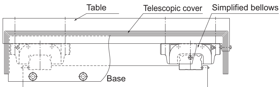
Fig.2 Example of Mounting the Simplified Bellows
