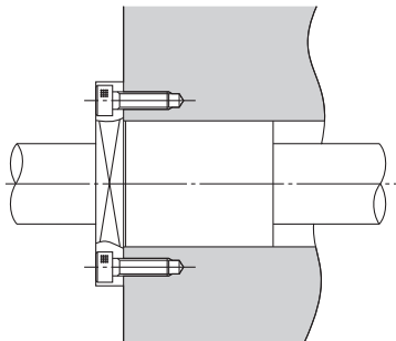
Nut mounted via socket and spigot joint
