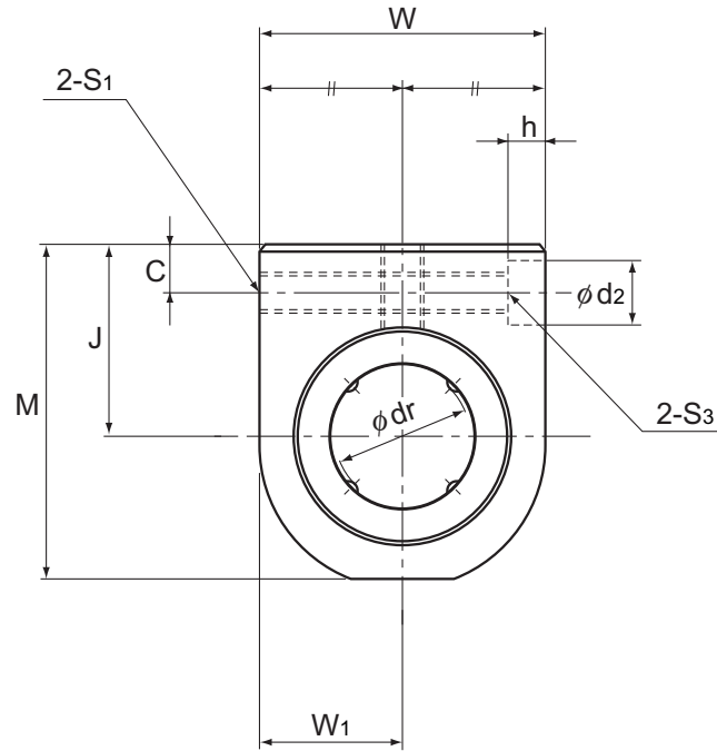
Model SH-L
