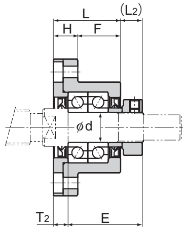
Mounting method B
