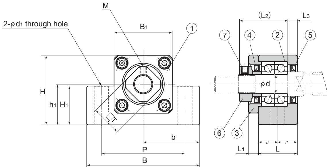
Models EK 10 to 20
