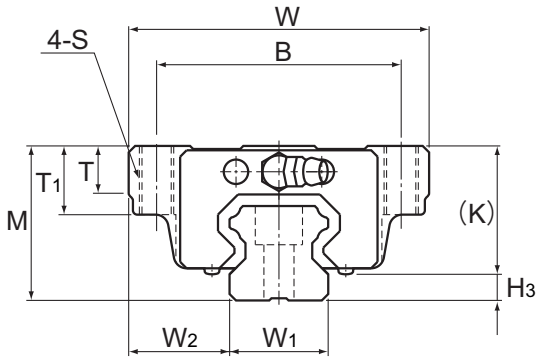
Models HSR15 to 35A/LA/AM/LAM
