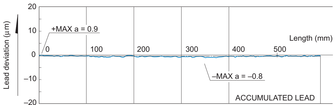
Fig.3 Lead Accuracy Measurement
