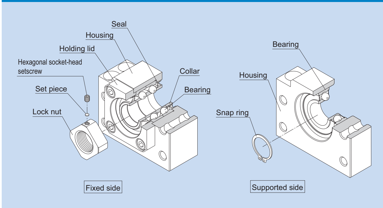
Fig.1 Structure of the Support Unit
