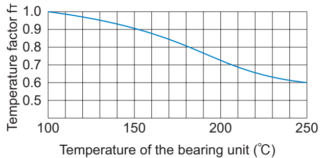
Fig.1 Temperature Factor ( f_T )
