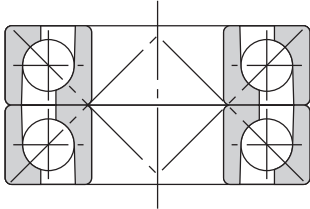
Angular Ball Bearings Mounted Front-to-front (DF type)
