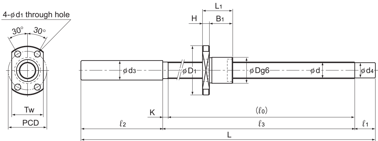
Model MDK
