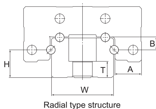
Fig.3 Cross Section of Model NR
