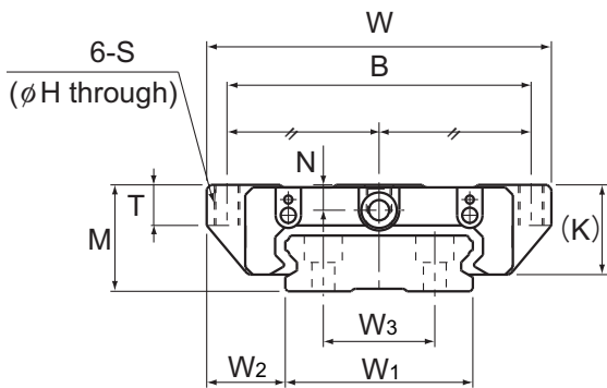
Models SHW17CAM and SHW21 to 50CA
