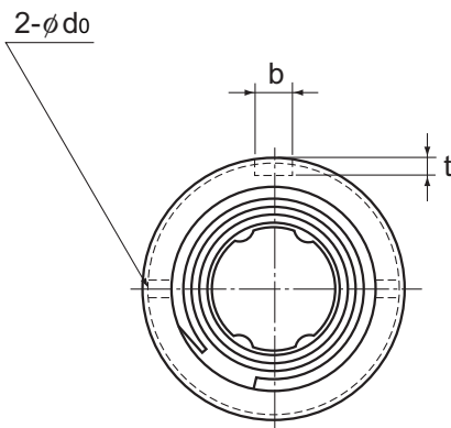
Model LT13 or smaller
