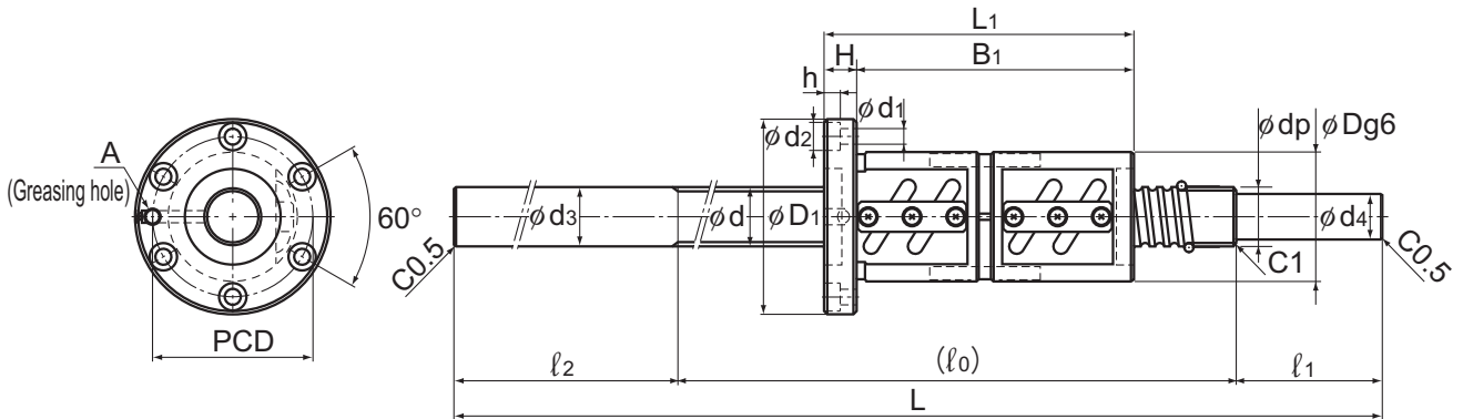
Model BNFN
