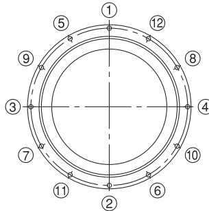
Fig.1 Tightening Sequence
