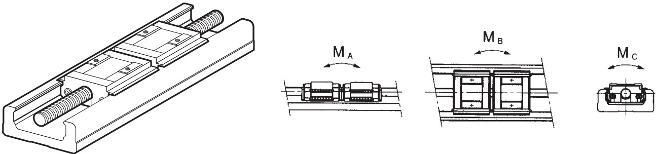
With double short nut blocks (type D)
