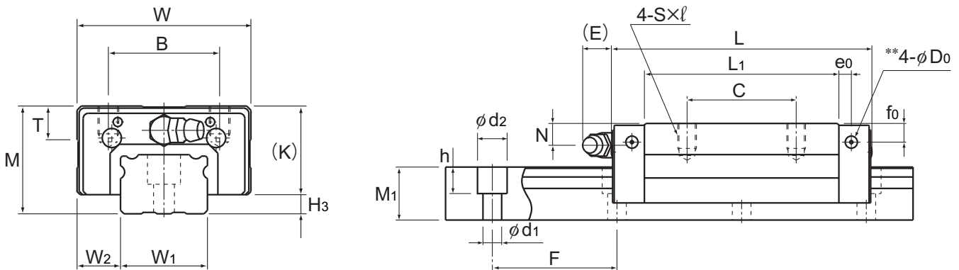
Model SNR-R
