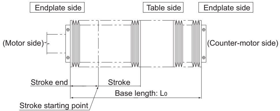
Fig.6 Schematic Drawing of Mounting the Bellows
