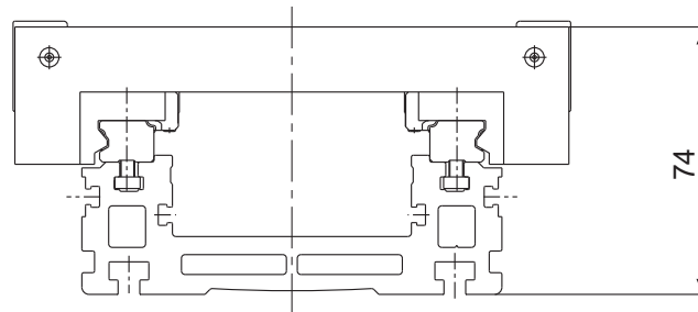
Fig.2 Mounting Height of the Bellows
