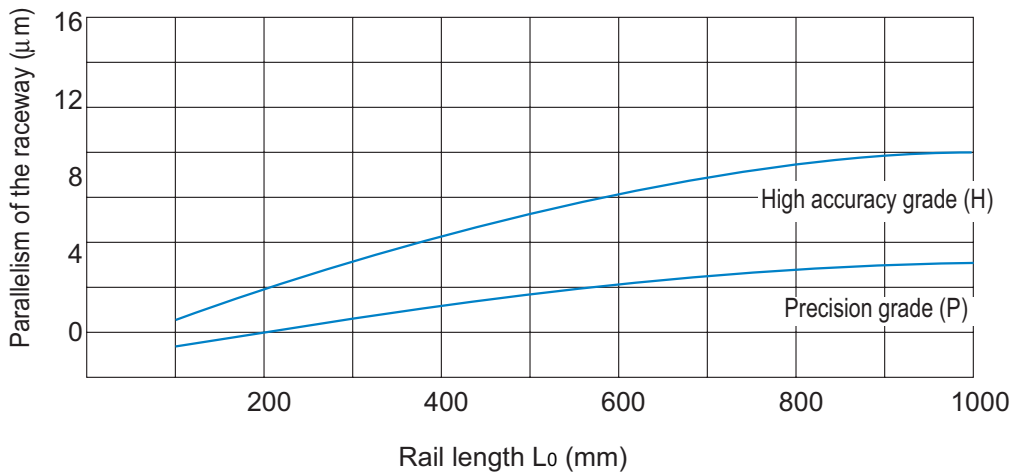
Fig.4 Rail Length and Parallelism of the Raceway
