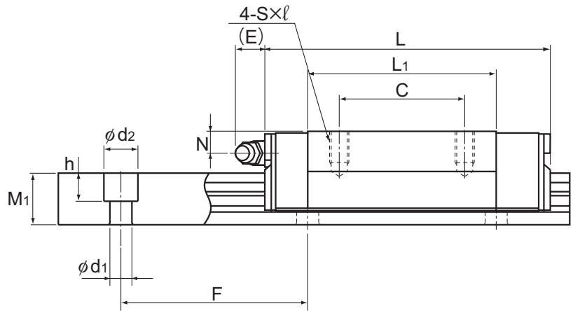
Models GSR15 to 35T
