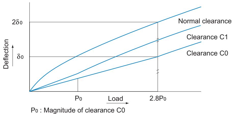
Fig.15 Rigidity Data
