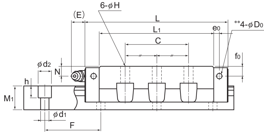
Model NR-LB
