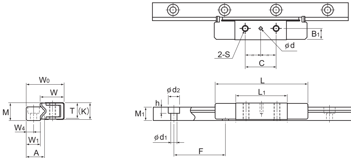
Models HR918 and 918M
