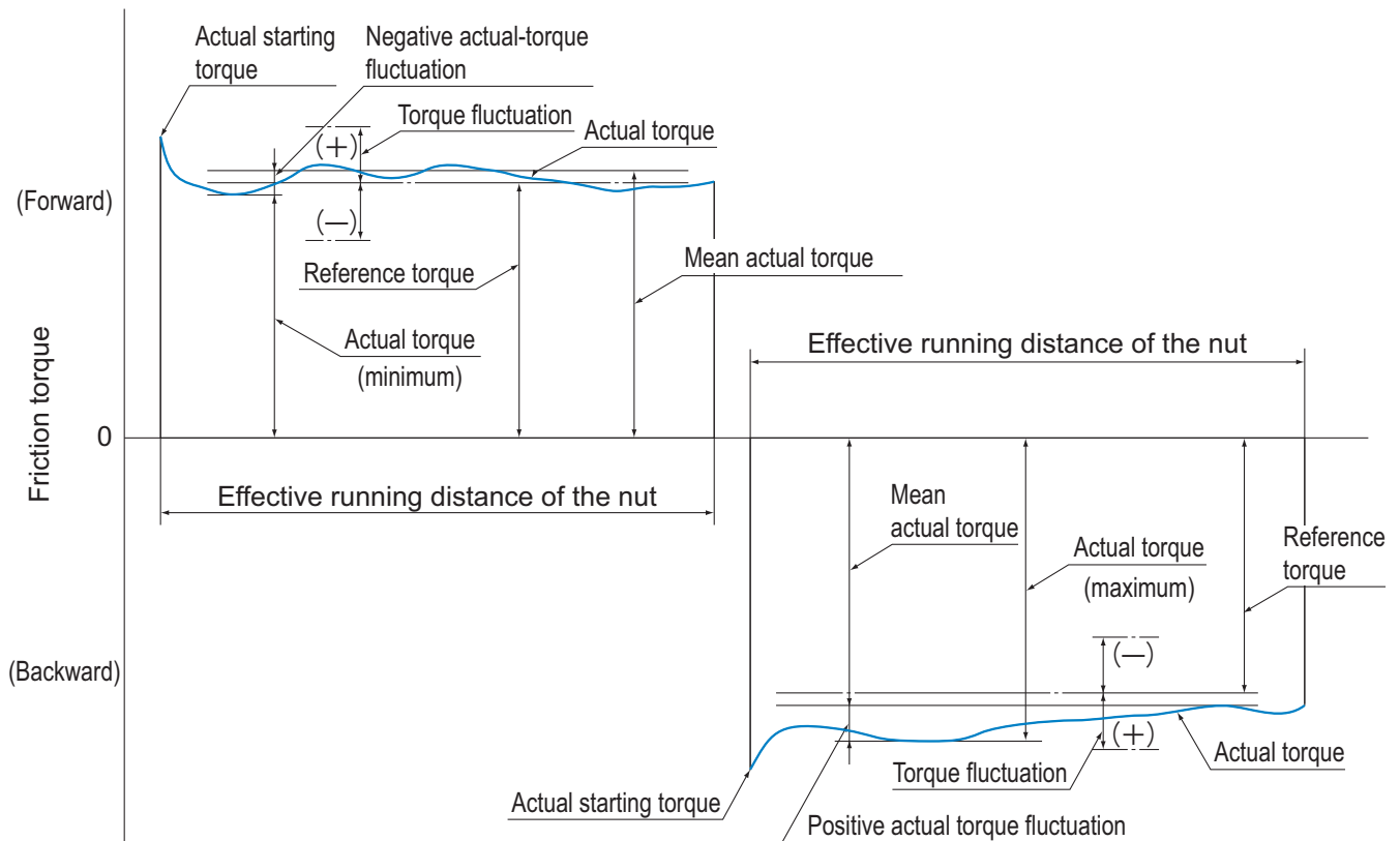
Fig.7 Terms on Preload Torque
