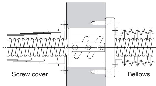
Contamination Protection Cover for the Ball Screw
