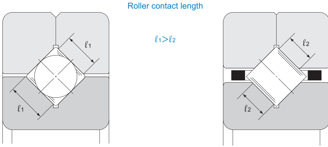
With a spacer retainer
