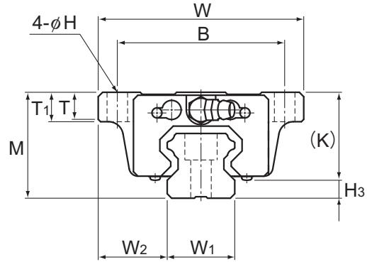
Models HSR20M1B/M1LB
