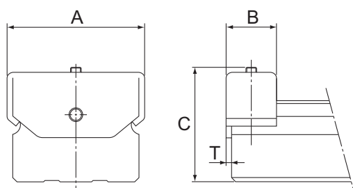
Fig.1 End Piece EP for Models NR/NRS
