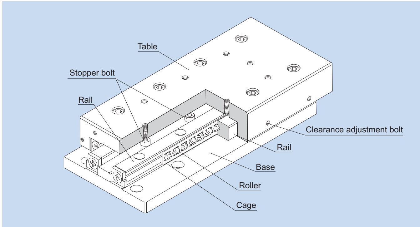
Fig.1 Structure of the Cross Roller Table
