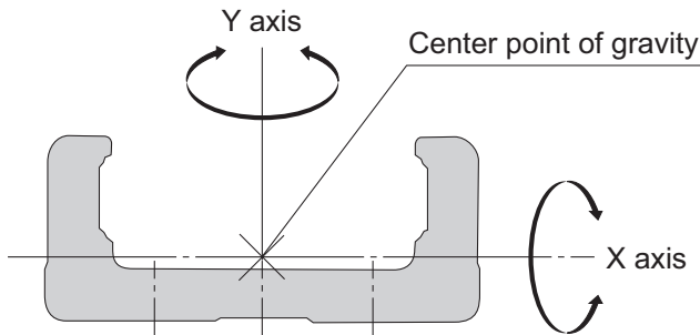
Fig.3 Cross Section of the LM Rail
