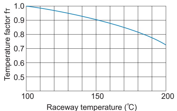
Fig.3 Temperature Factor ( f_T )
