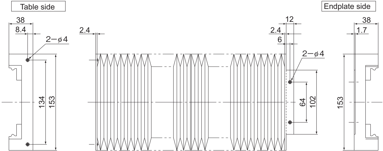
Fig.1 External Dimensions of the Bellows
