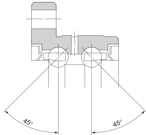
Fig.1 Structure of the Support Bearing
