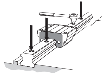
Fig.6 Fully Fastening the Mounting Bolts
