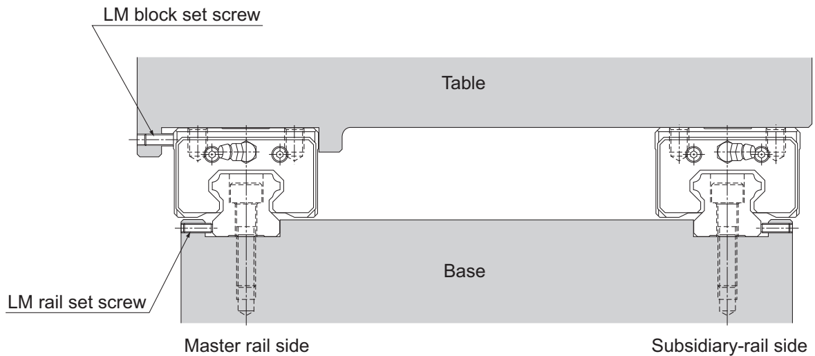
Fig.1 When the Machine Receives Vibrations or Impact
