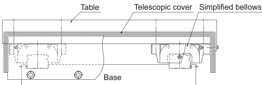
Fig.1 Example of Mounting the Simplified Bellows
