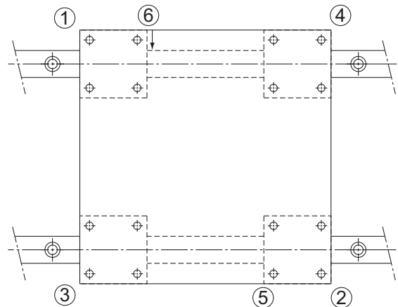
Fig.7 Sequence of Tightening the LM Blocks
