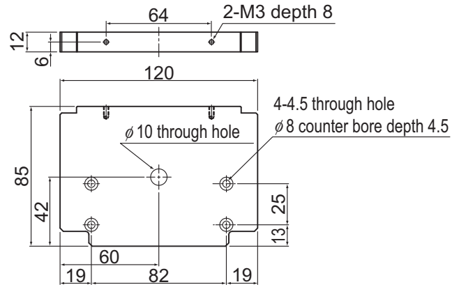
Model GL20
