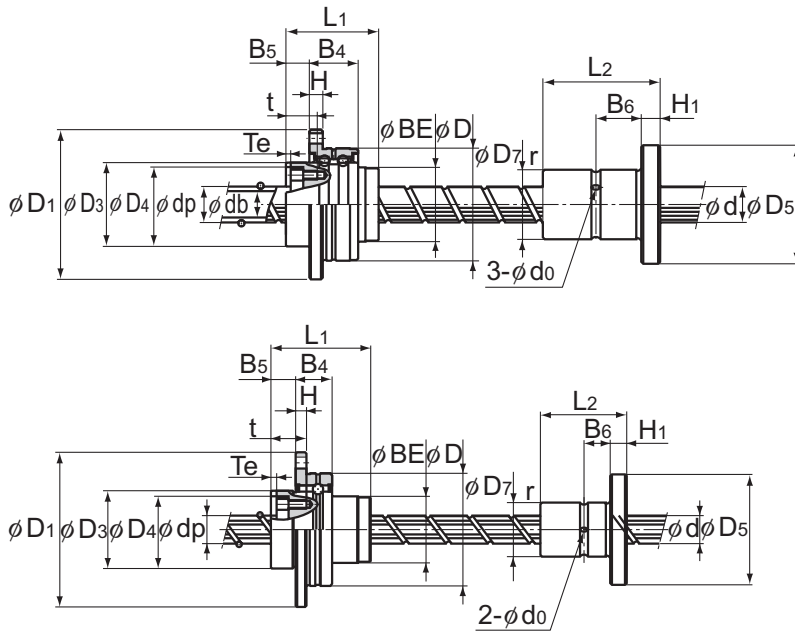
Models NS 0812A and 1015A
