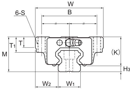
Models HSR20 to 35CA/HA/CAM/HAM
