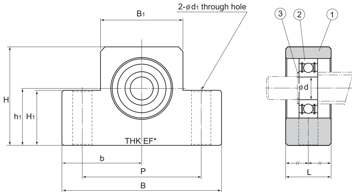
Models EF 10 to 20
