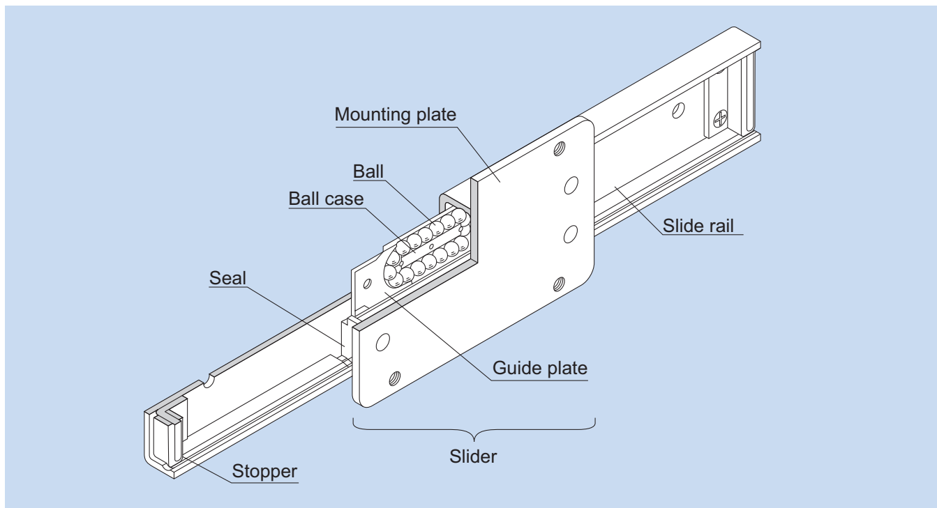
Fig.1 Structure of Slide Pack Model FBW-RUU
