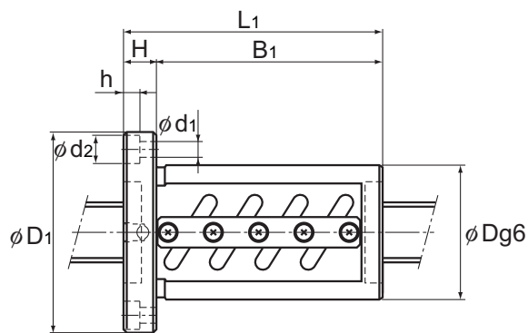
Model BIF
