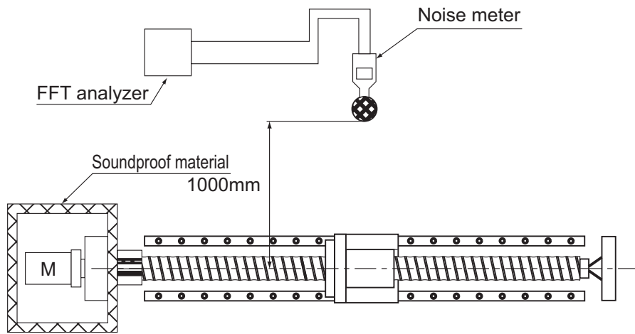
Noise measurement instrument
