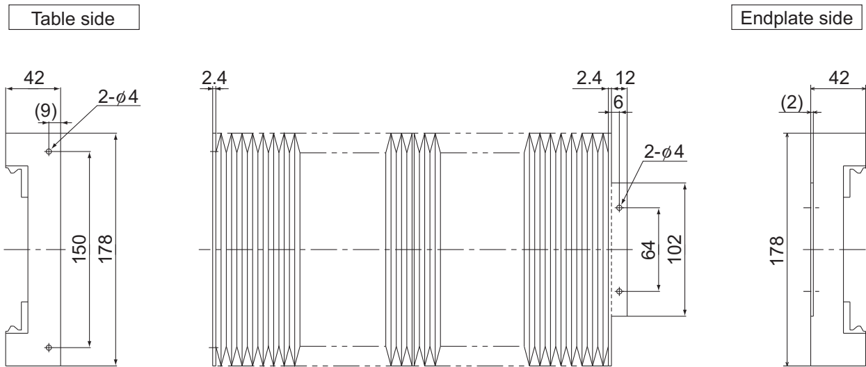
Fig.4 External Dimensions of the Bellows
