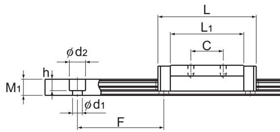
Models SHW12CRM, SHW12HRM and SHW14CRM
