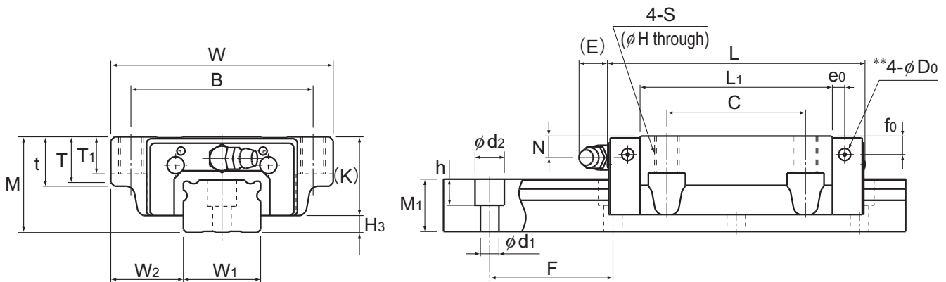
Model SNS-C
