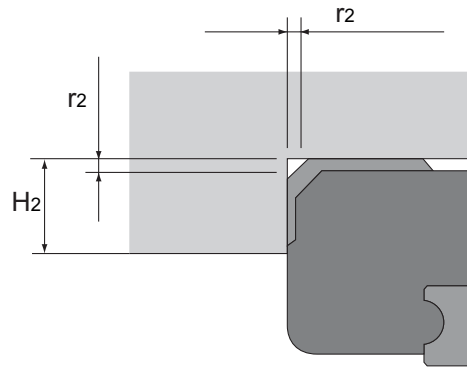
Shoulder for the LM Block
