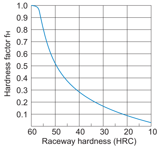
Fig.11 Hardness Factor ( f_H )
