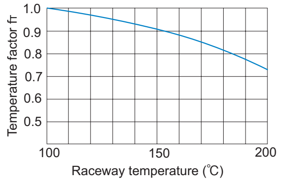
Fig.1 Temperature Factor (f r )
