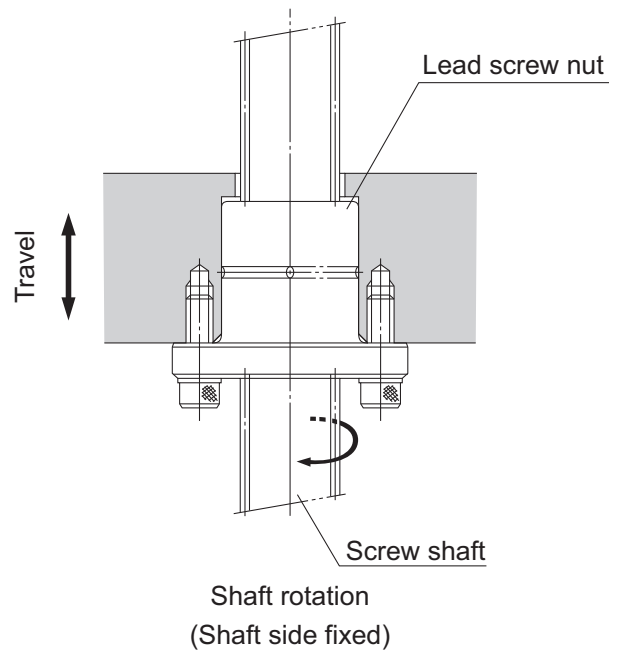
Fig.2 Recommended Mounting Orientation
