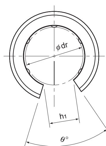
Model LME-OP
