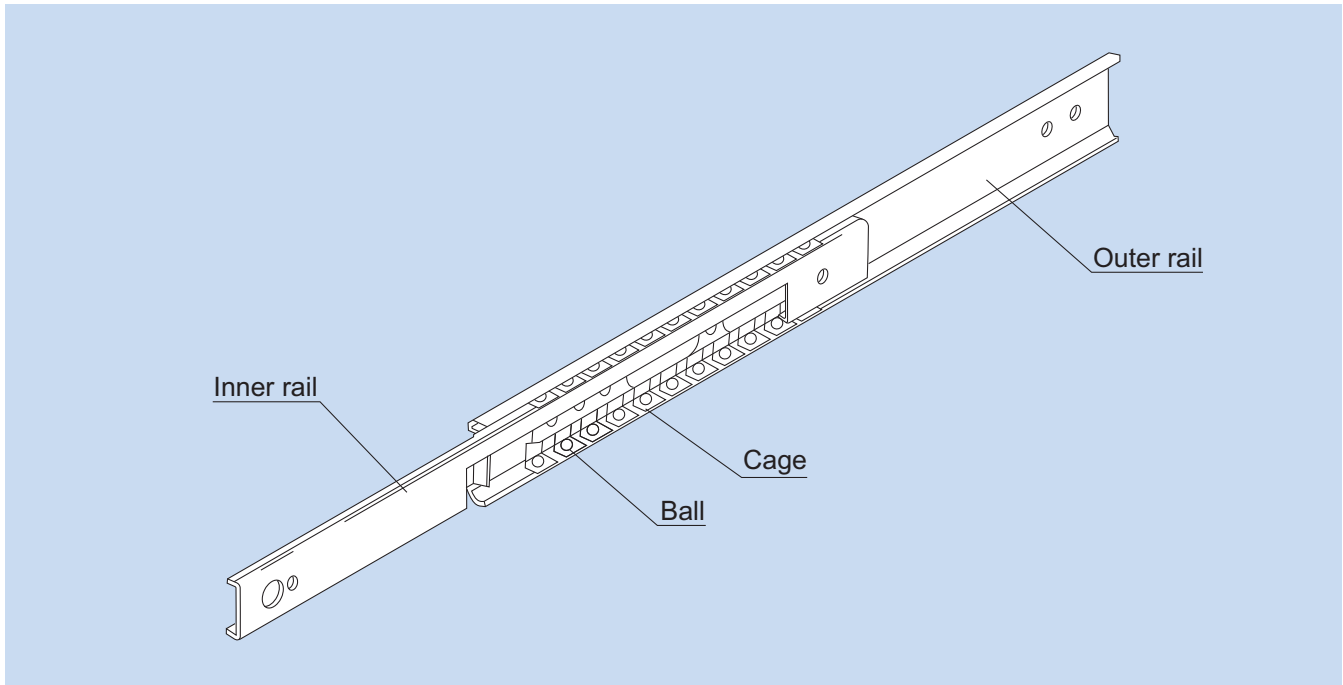
Fig.1 Structure of Slide Rail Model FBL
