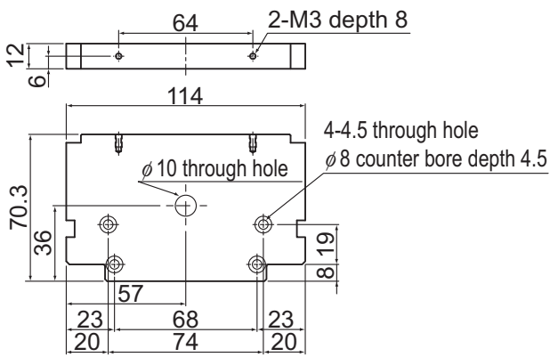
Model GL15
