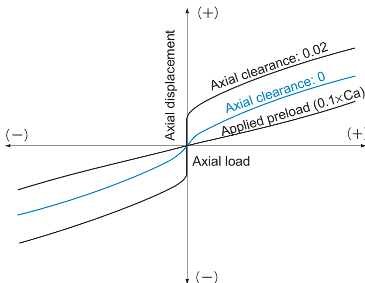
Fig.6 Axial Displacement in Relation to Axial Load
