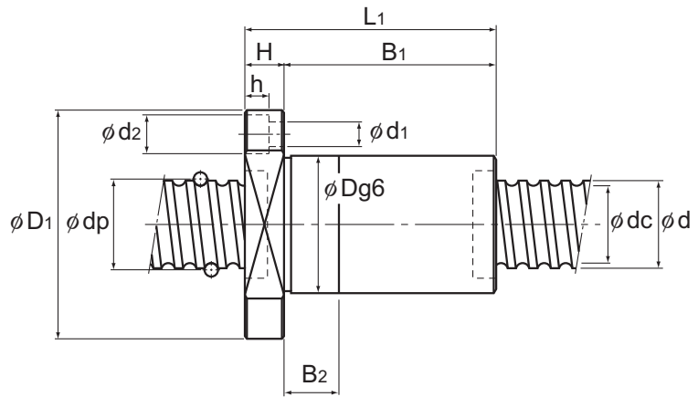
DIK (2805 to 6312)
