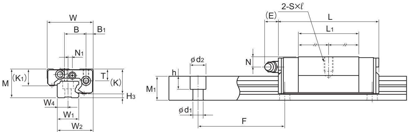
Model GSR15T/V
