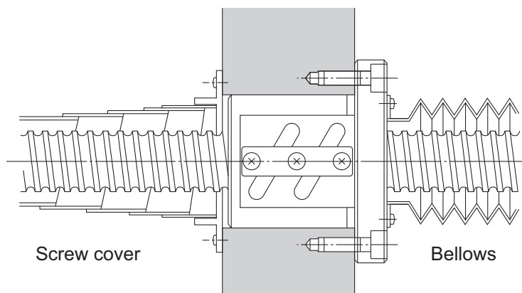
Fig.1 Contamination Protection Cover
