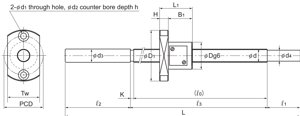
Model MBF
