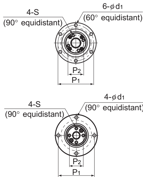
Models NS 0812A and 1015A
