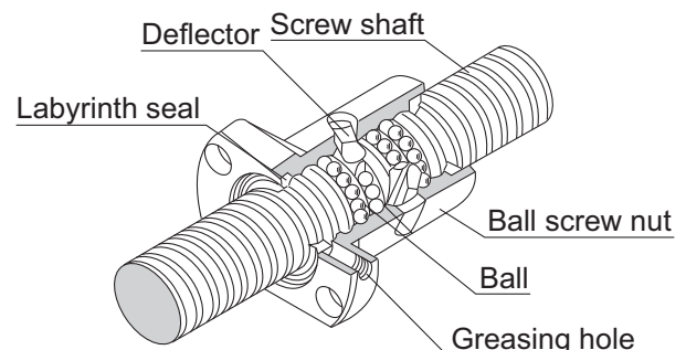
Example of Structure of Simple Nut
