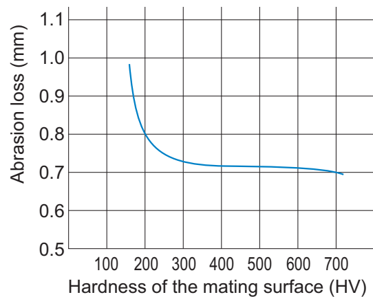
Fig.3 Hardness of the Surface and Wear Resistance
