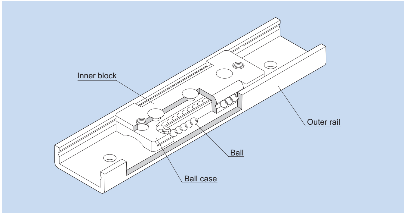
Fig.1 Structure of Precision Linear Pack Model ER
