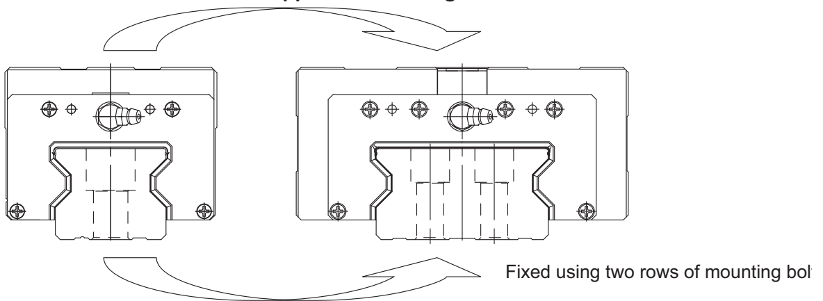
Fig.2 Comparison between Models SRW and SRG in Cross Section
