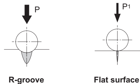
Fig.2 Load Capacity per Ball
