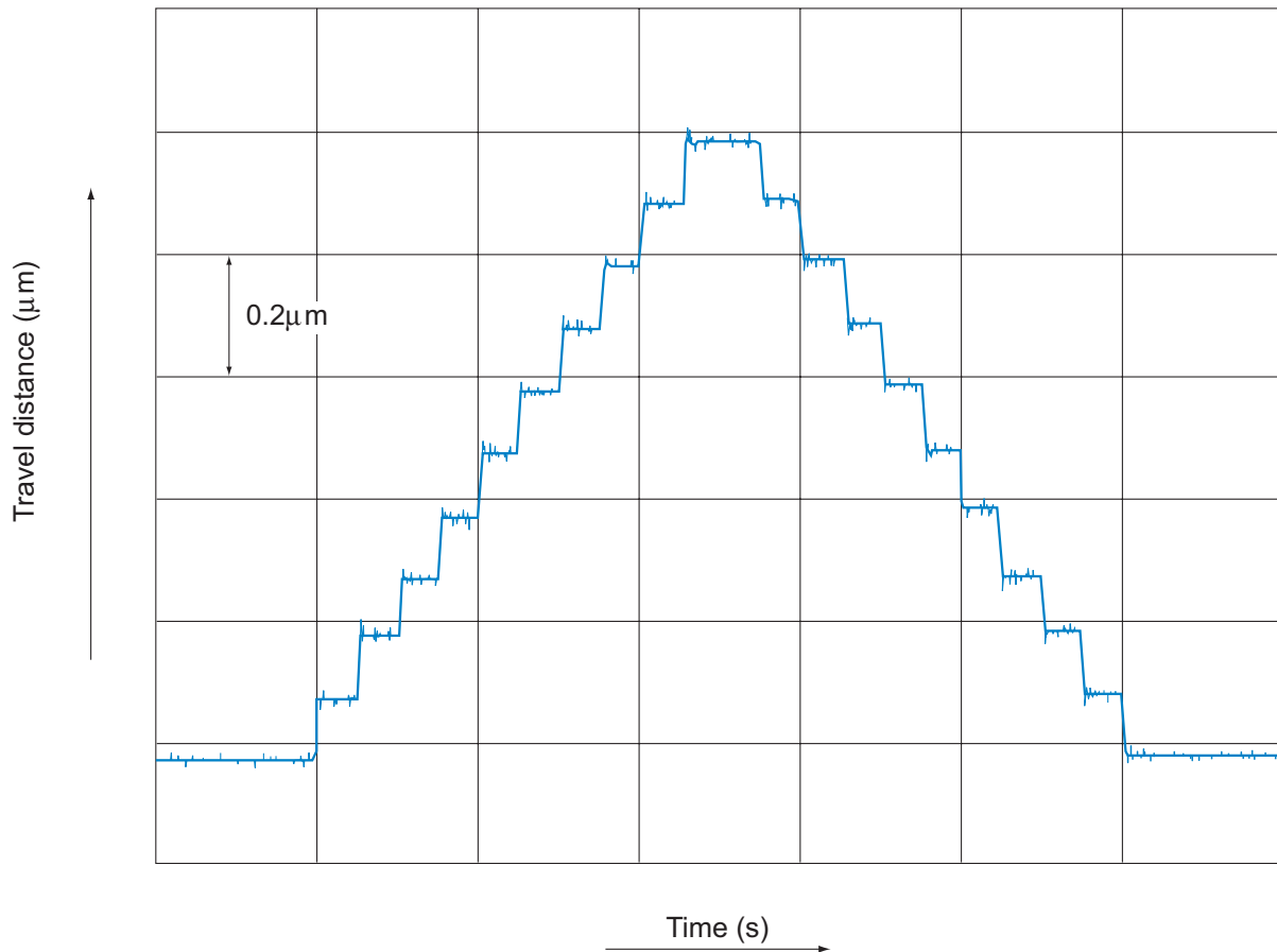
Fig.4 Data on Travel in 0.1- \mu\text{m} Feeding
