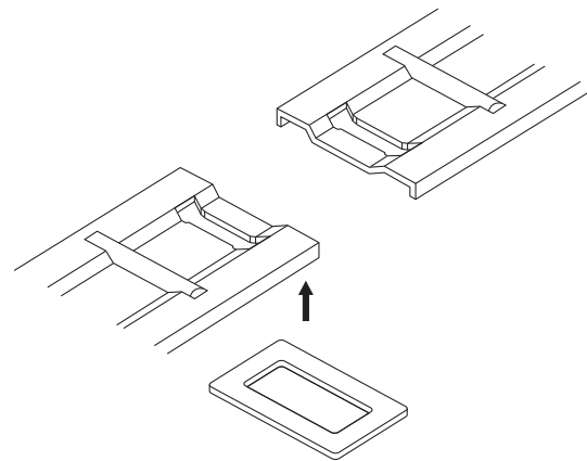
Fig.4 Connection of Model FT Units
