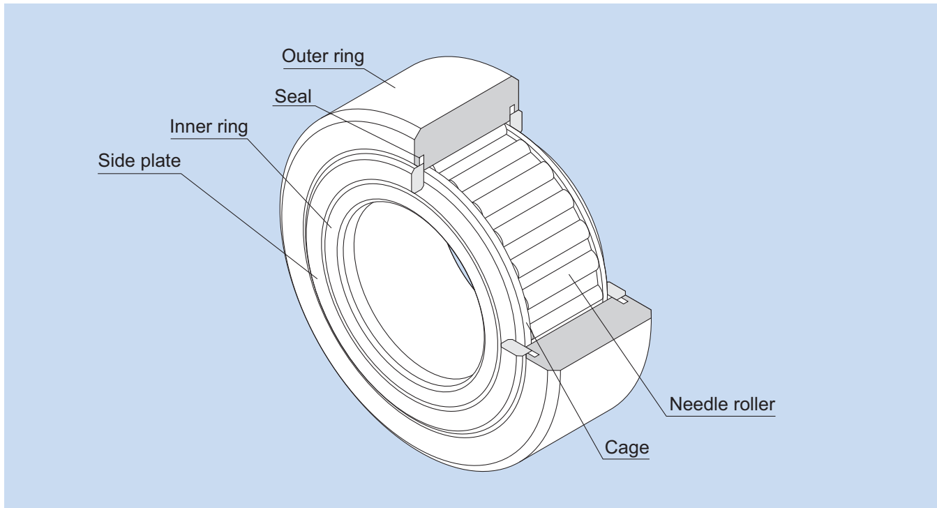
Fig.1 Structure of Roller Follower Model NAST-ZZUU
