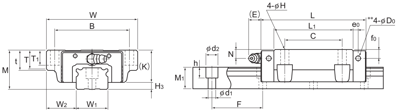
Model NR-B
