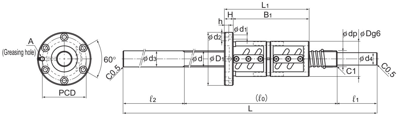
Model BNFN
