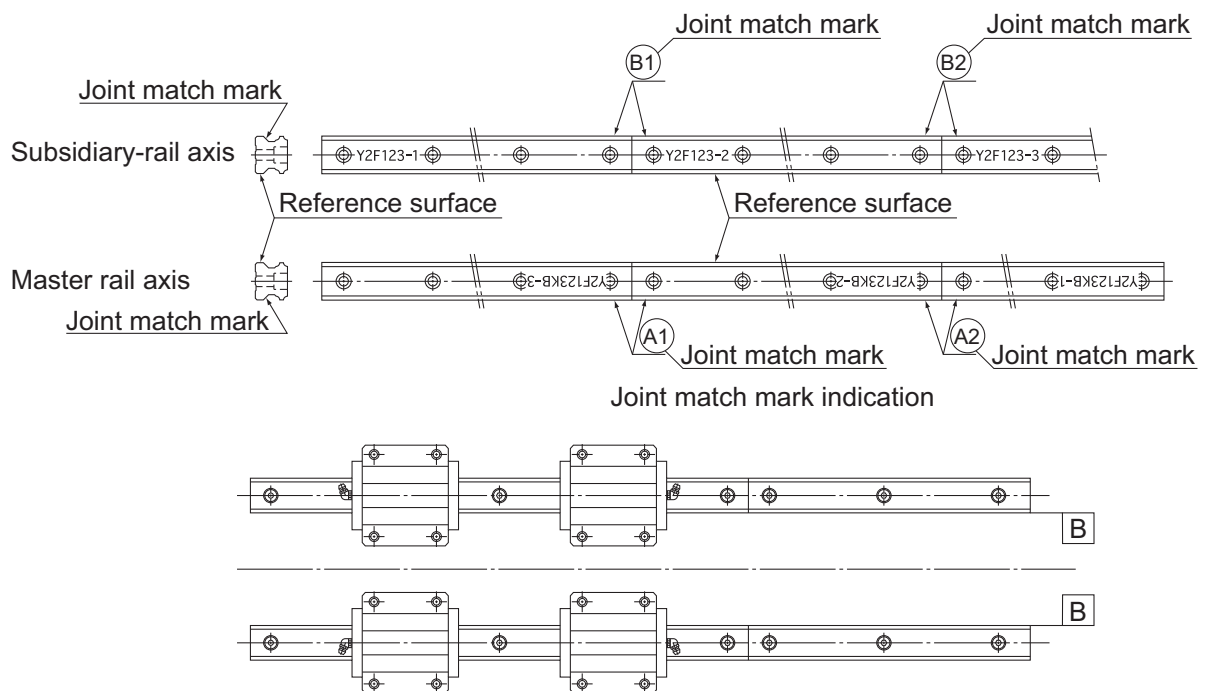
Fig.23 Use of Jointed Rails
