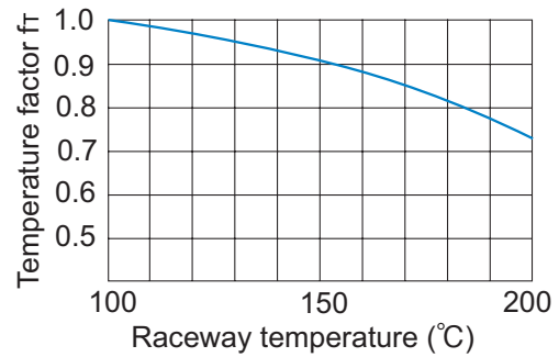
Fig.1 Temperature Factor ( f_T )
