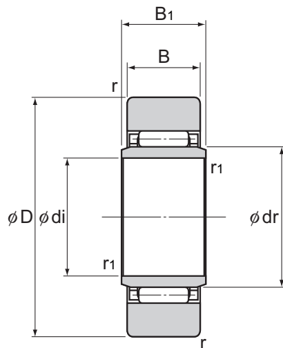
Model NAST
