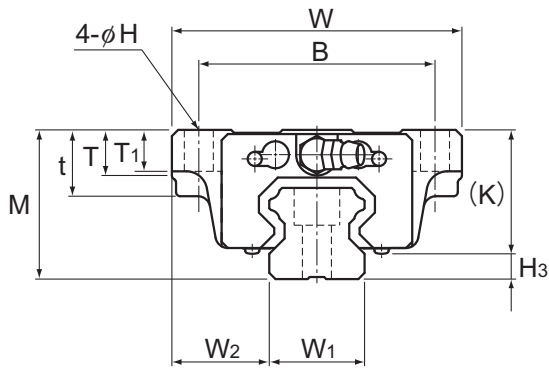
Models HSR15, 25 to 35M1B/M1LB
