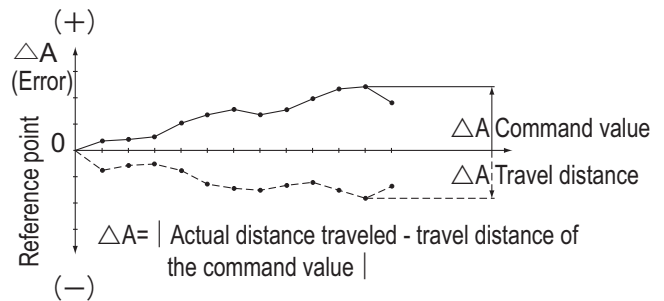
Fig.10 Positioning Accuracy
