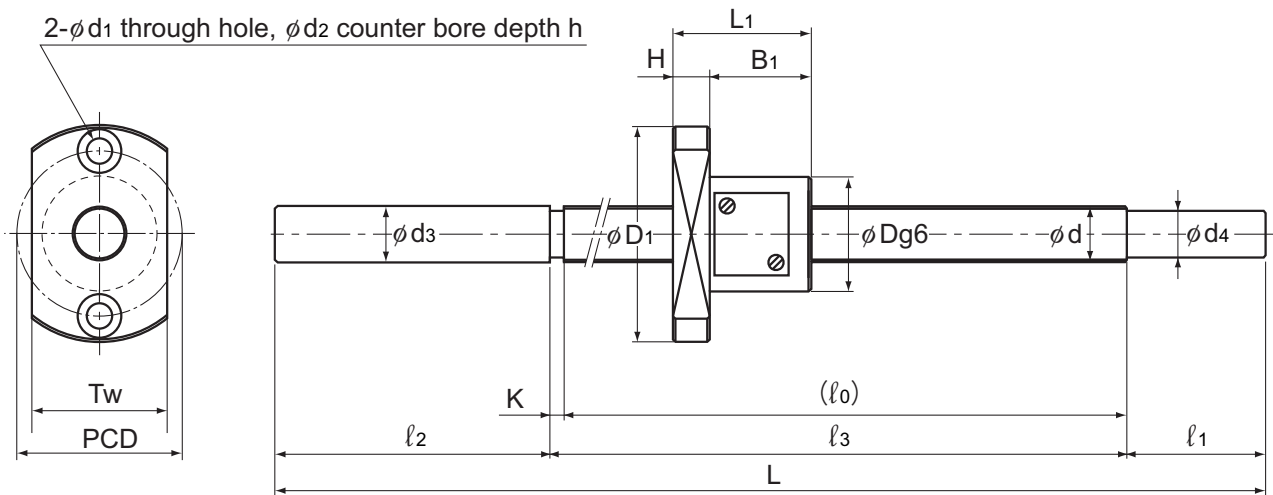
Model MBF
