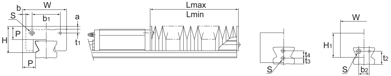
Models SR15 to 25 Models SR30 to 70
