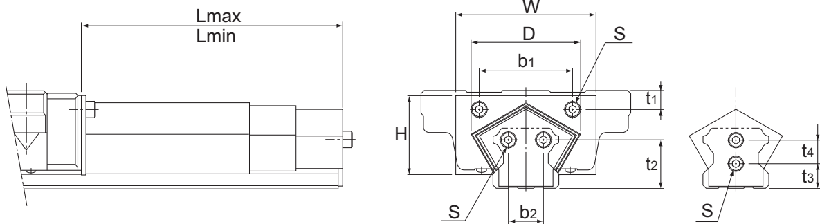
Models HSR25 and 30
