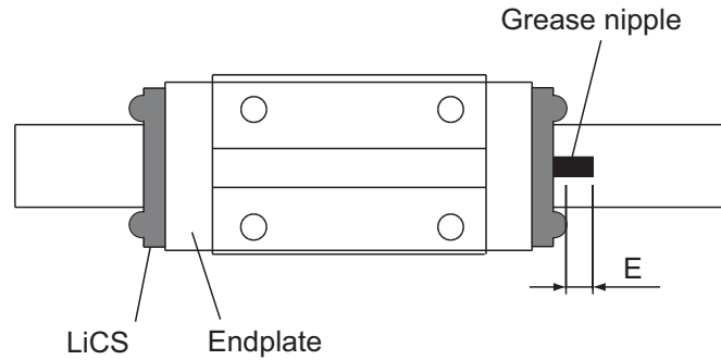
Location for Mounting the Grease Nipple
