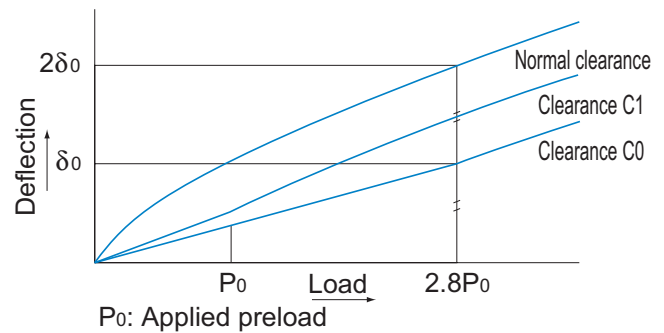
Fig.5 Rigidity Data
