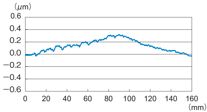
Fig.5 Dynamic Accuracy of a Single-axis Table
