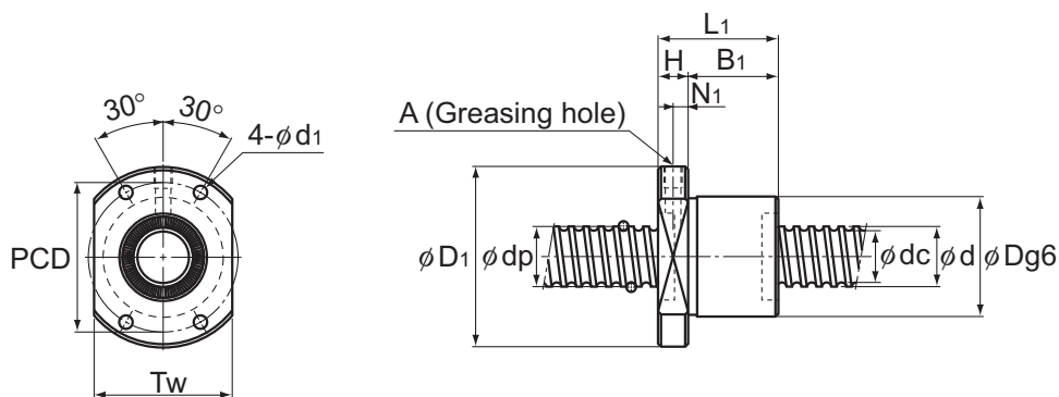
Models BTK 1404 to 5016
