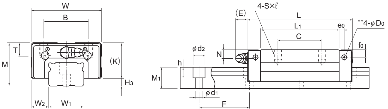
Model SNS-R
