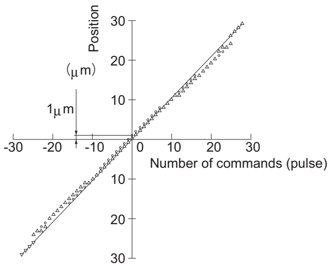
LM Guide model HSR45
