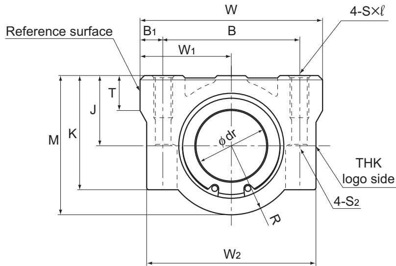
Models SC35 to 50
