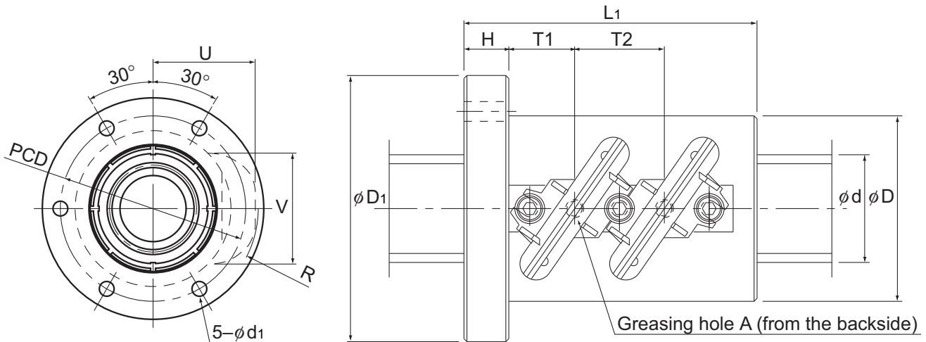
Models HBN3210 to 3612
