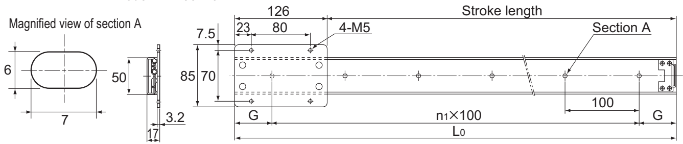
Model FBW50110R
