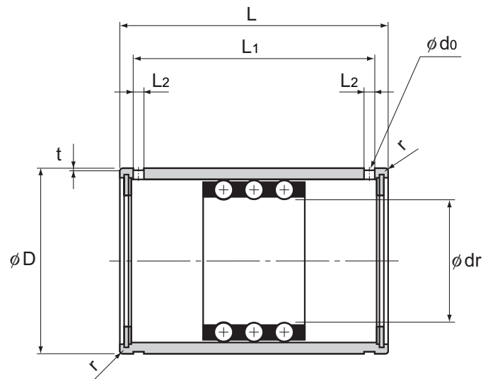
Model ST (For light load)
