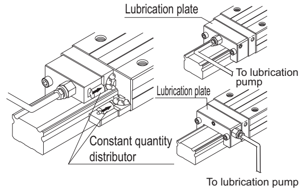
Fig.3 Structural Drawing
