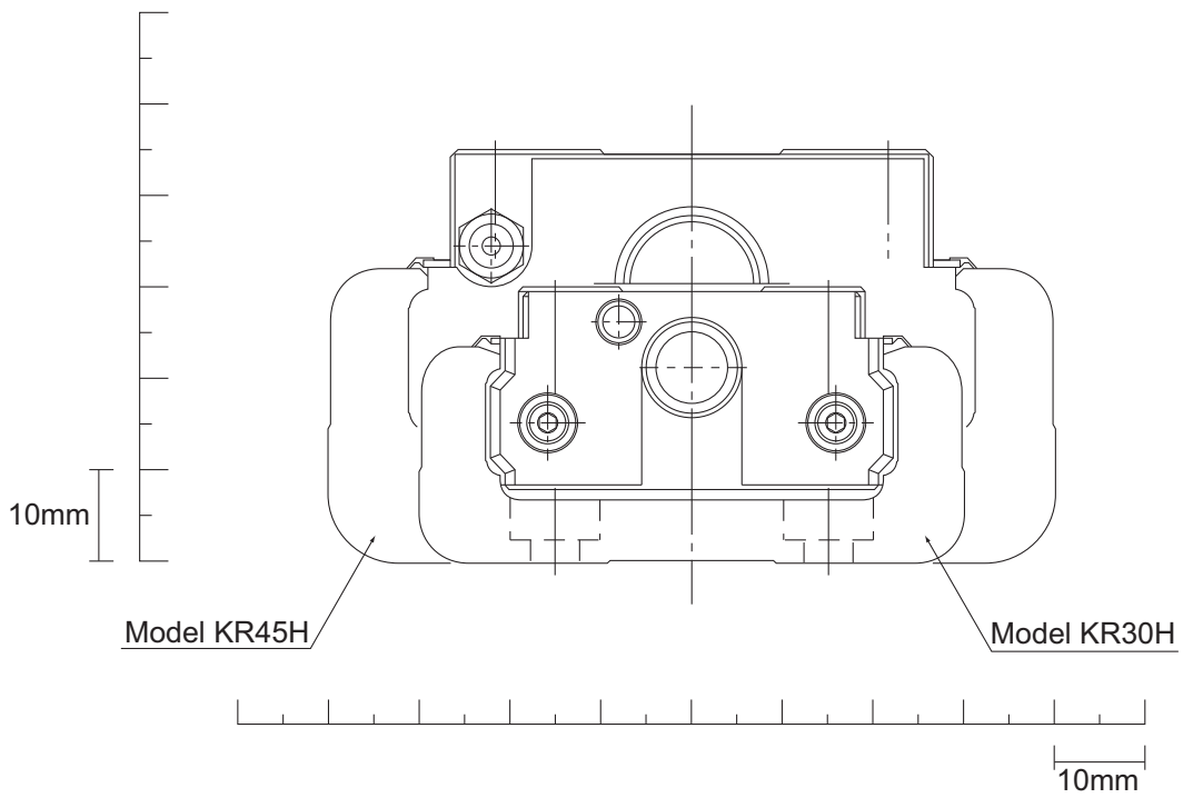
Fig.6 Cross Sectional Drawing
