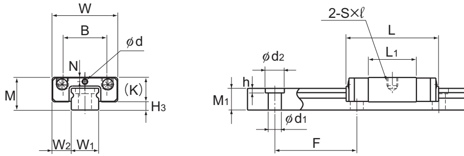
Model RSR5M
