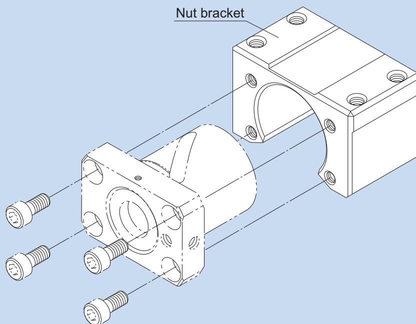
Fig.1 Structure of the Nut Bracket
