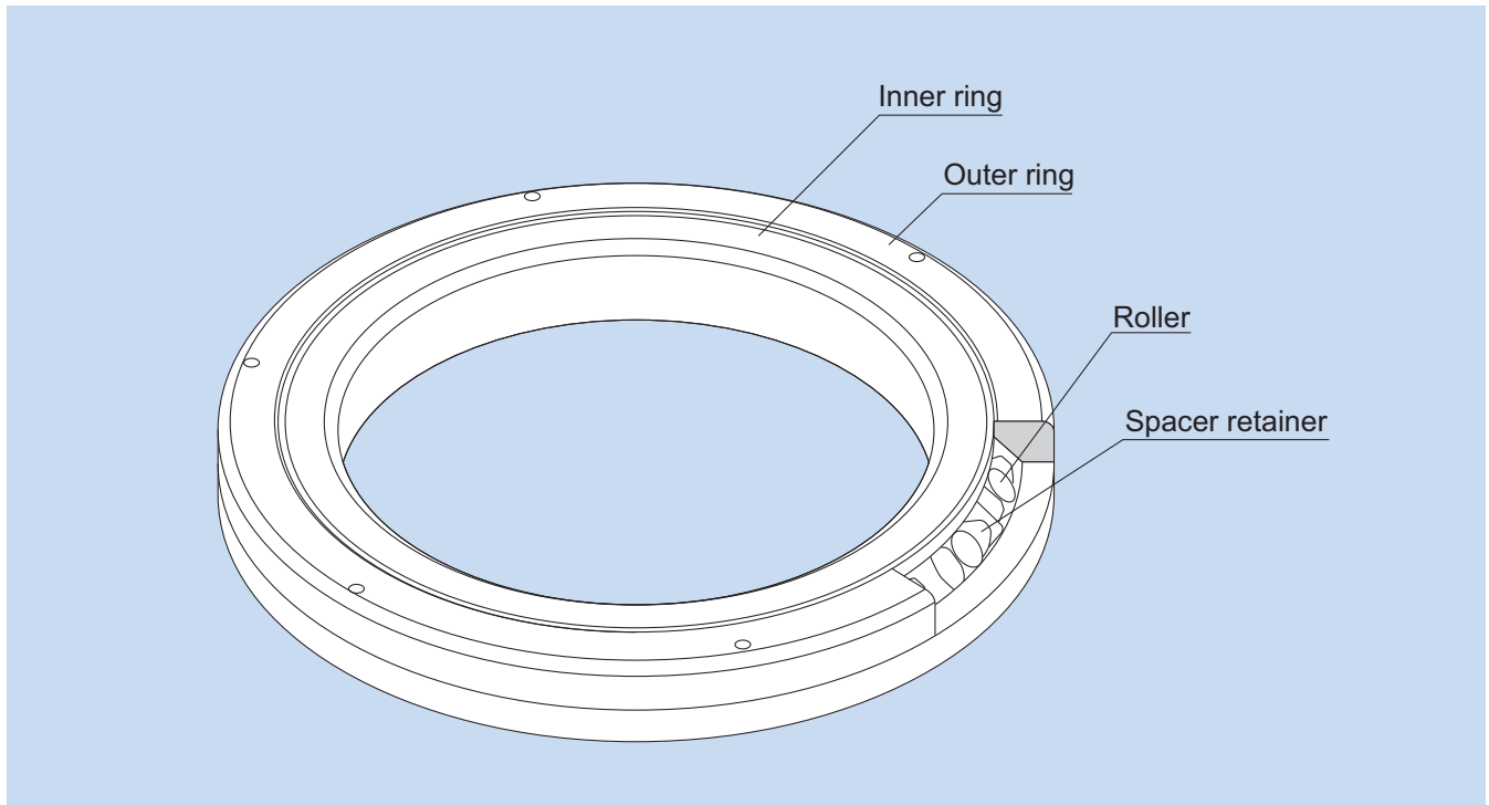
Fig.1 Structure of Cross Roller-Ring Model RB
