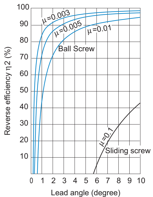
Fig.2 Reverse Efficiency (Linear to Rotational)
