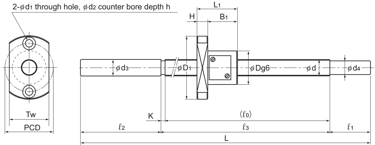
Model MBF
