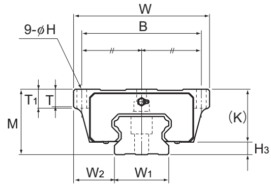
Models HSR100 to 150HB
