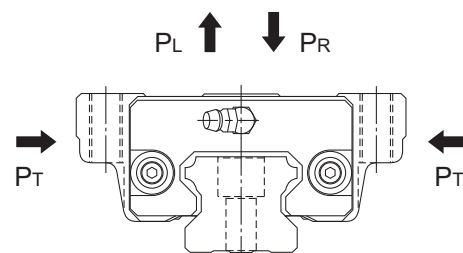
Fig.1 Model HSR-M2
