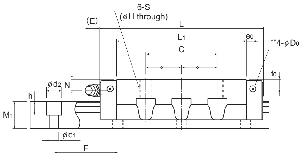
Model SNS-LC
