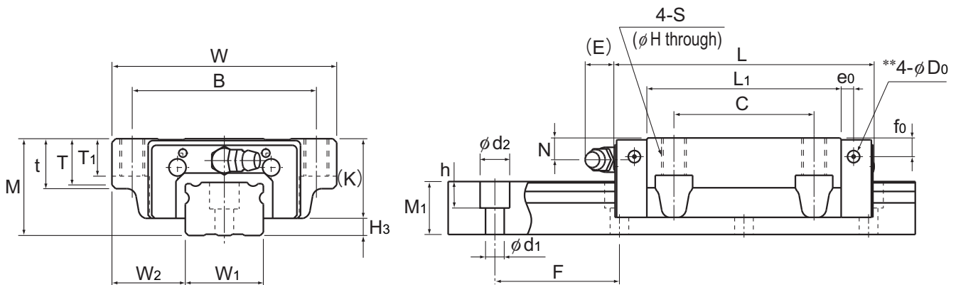
Model SNR-C
