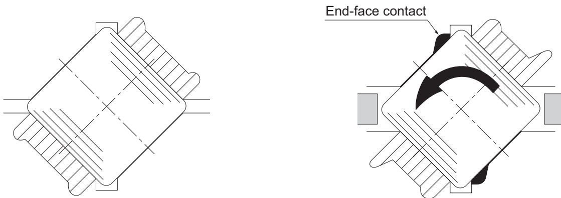
Loaded areas symmetrical With a spacer retainer
