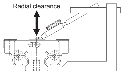
Fig.3 Radial clearance of the LM Guide
