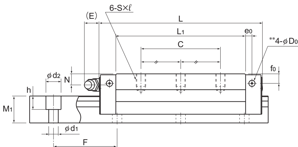
Model SNR-LR
