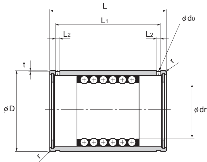
Model ST-B (For medium load)
