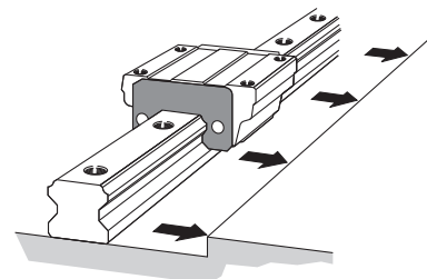
Fig.3 Aligning the LM Rail with the Reference-Surface
