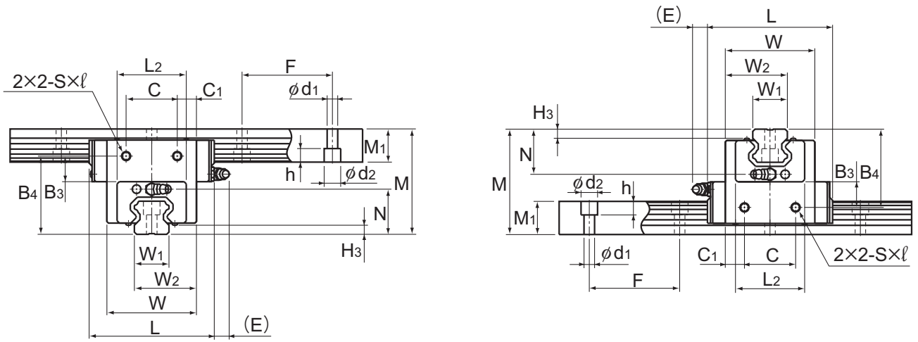
Models CSR15, 20S to 30S
