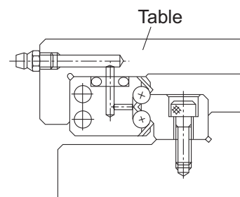
Fig.3 Example of Machining a Greasing Hole
