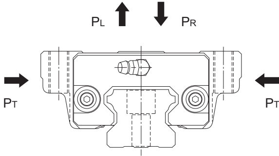
Fig.3 Model HSR-M1
