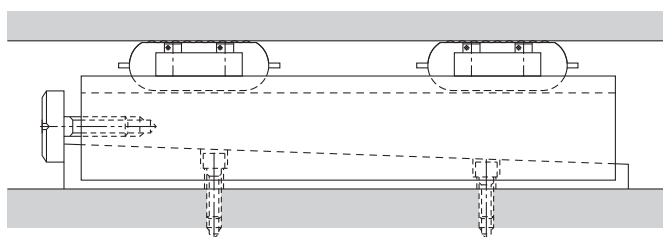
(c) Adjusting a tapered gib
