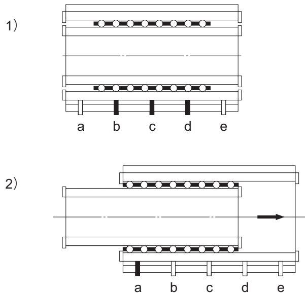
Fig.2 Sequence of Tightening the Adjustment Bolts
