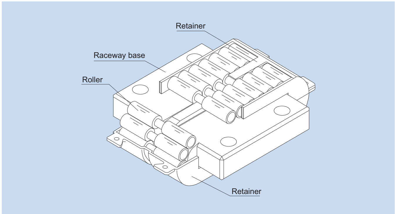
Fig.1 Structure of LM Roller Model LR
