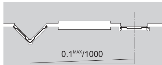
Fig.2 Mounting Precision
