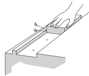
Fig.2 Checking the Mounting Surface
