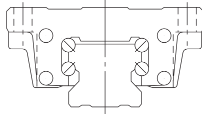
DF Type Four-row Angular Contact (LM Guide)
