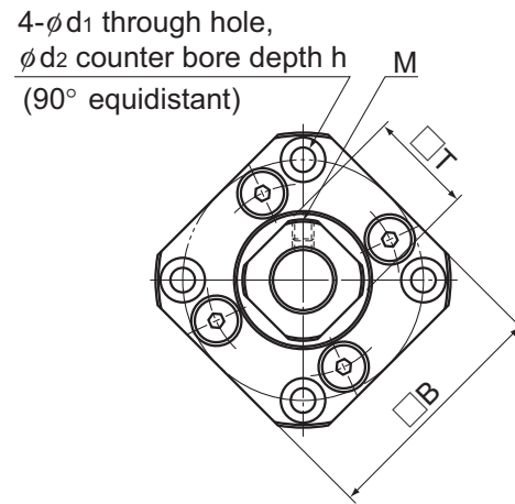
Models FK 10 to 30
