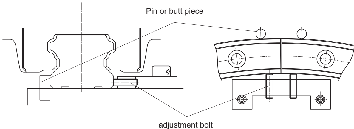
Fig.1 Flush piece
