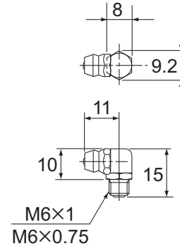
C-M6F (M6×0.75)
