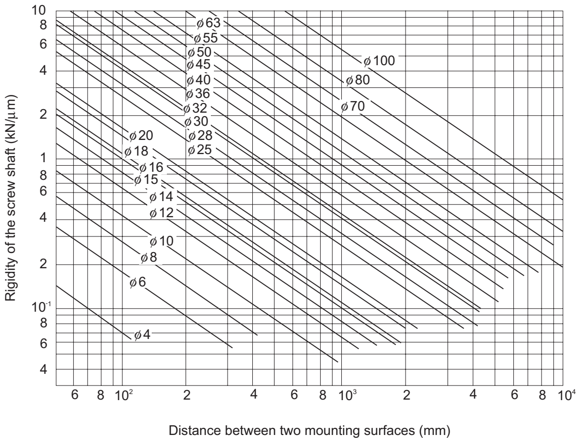
Fig.11 Axial Rigidity of the Screw Shaft (Fixed-Fixed)
