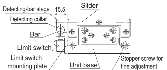
Fig.3 Unit Base and Limit Switch Installation
