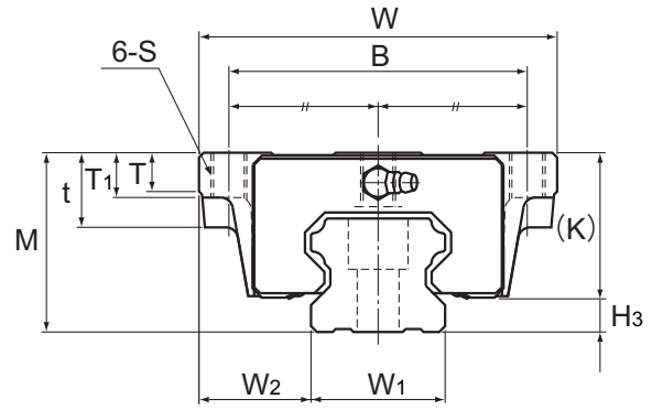
Models HSR45 to 85CA/HA
