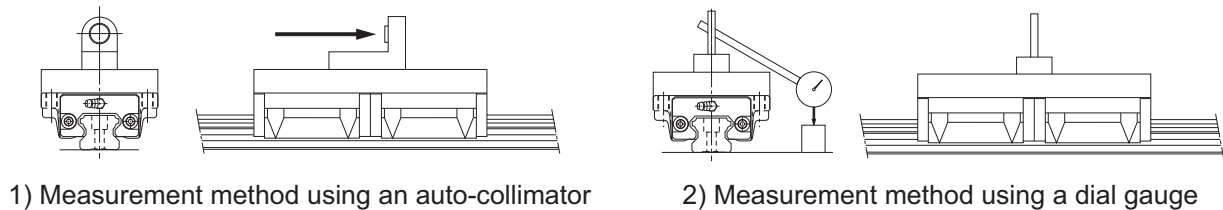
Fig.31 Methods for Measuring Accuracy after Installation
