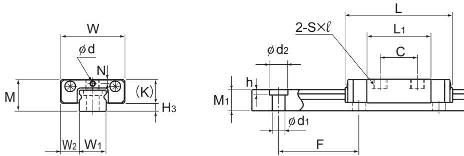
Model RSR5N
