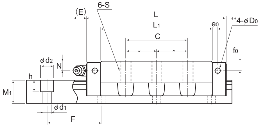
Model NRS-LA
