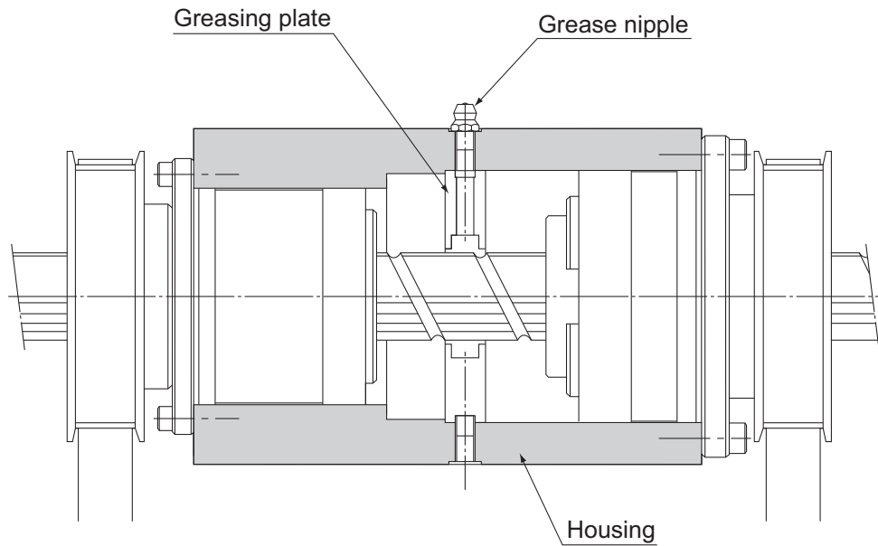
Fig.6 Lubrication Methods
