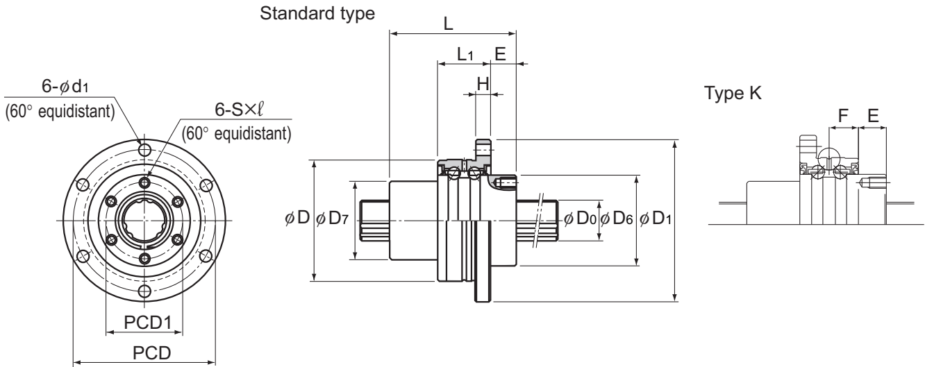
Model LTR16A or greater
