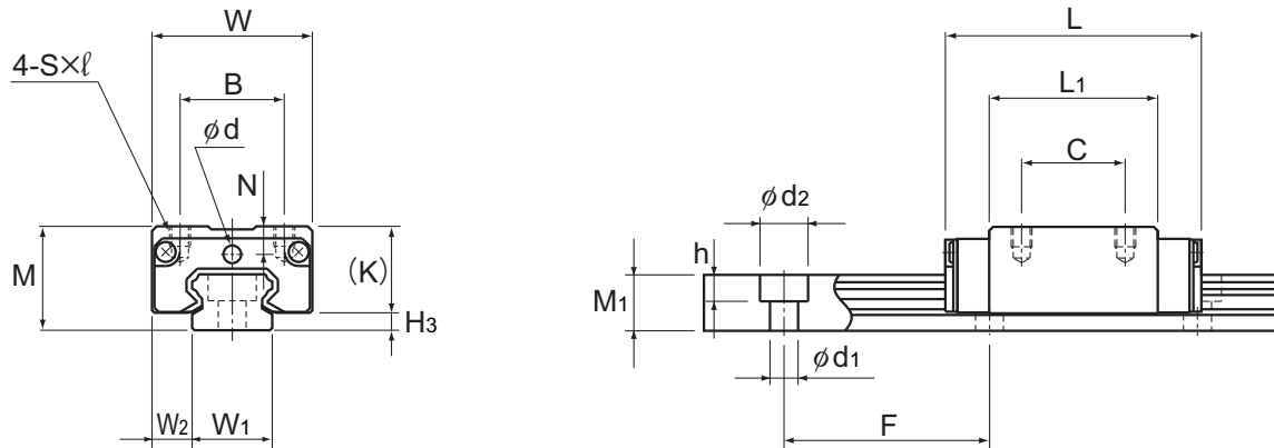
Models HSR8RM and 10RM
