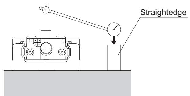
Fig.11 Running of Parallelism
