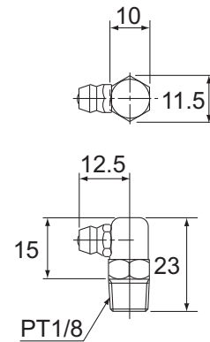
C-PT1/8
