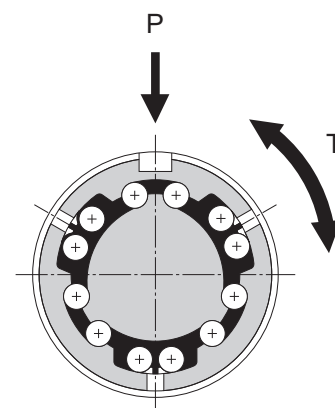
Fig.4 Angular backlash of the Ball Spline
