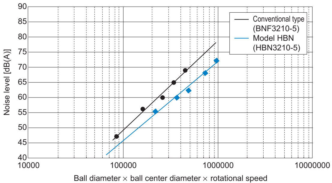
Fig.2 Ball Screw Noise Level
