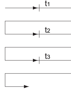
Fig.9 Positioning Repeatability
