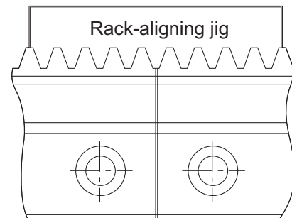
Fig.2 Rack Connection Method
