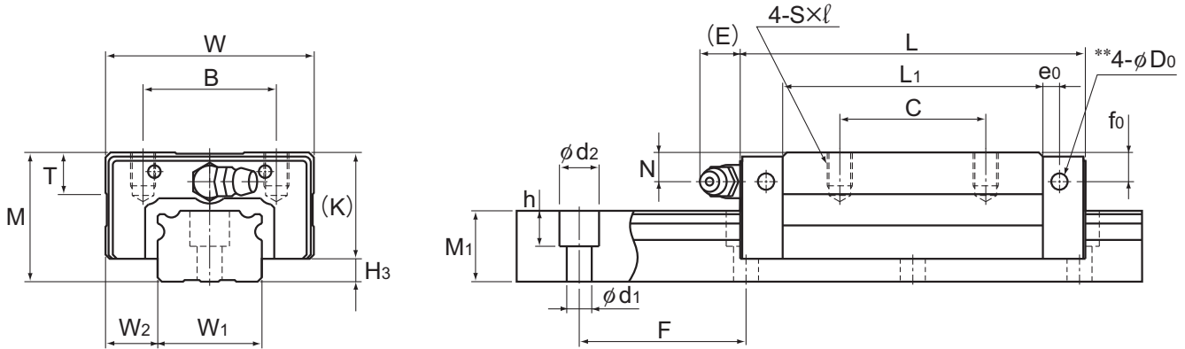
Model NRS-R
