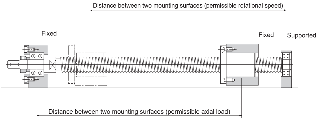
Fig.2 Screw Shaft Mounting Method: Fixed - Supported
