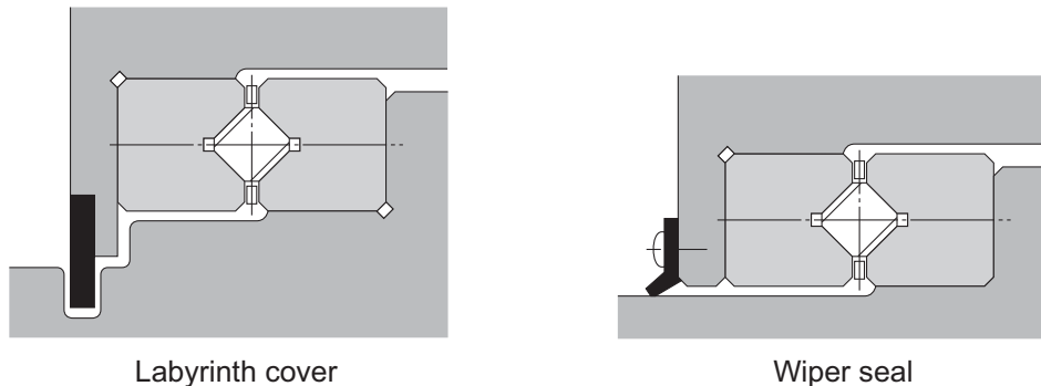
Fig.1 Contamination Protection Methods
