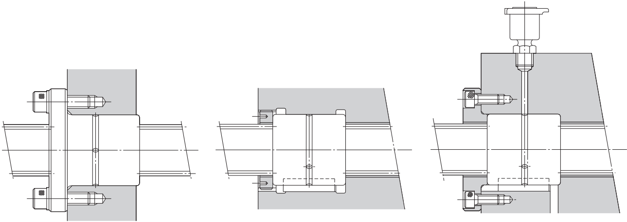
Fig.3 Examples of Installing the Lead Screw Nut
