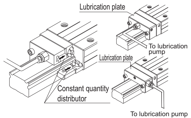
Fig.1 Structural Drawing
