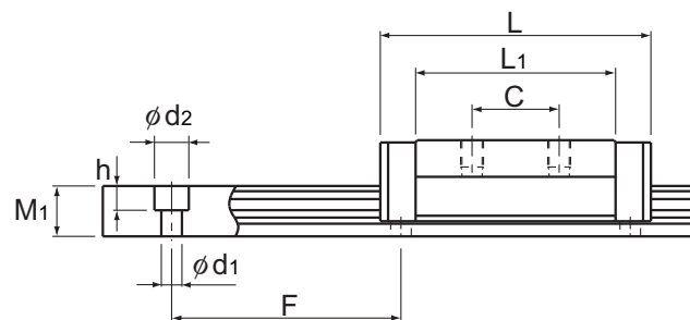
Models SHW17CRM and SHW21CR
