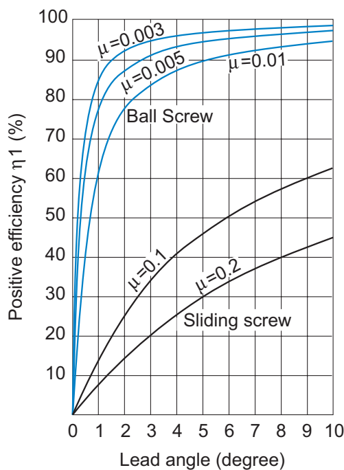
Fig.1 Positive Efficiency (Rotational to Linear)
