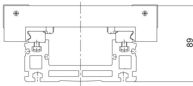
Fig.5 Mounting Height of the Bellows
