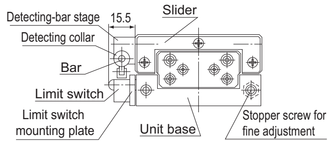
Fig.2 Unit Base and Limit Switch Installation
