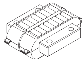
Model LR
