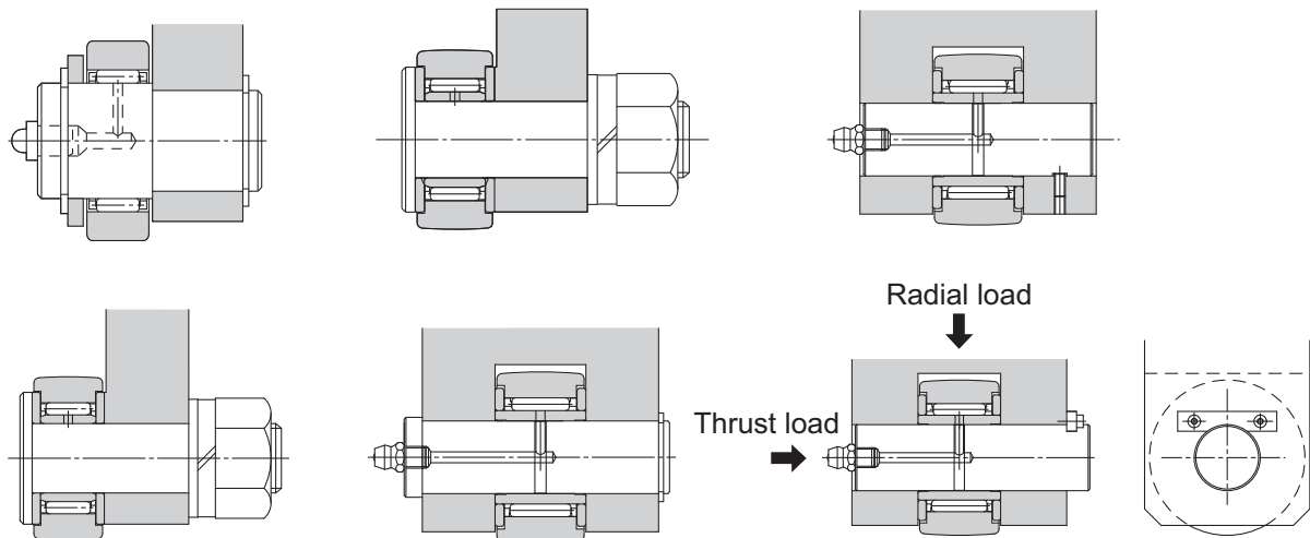
Fig.1 Examples of Installing the Roller Follower
