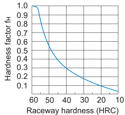
Fig.2 Hardness Factor ( f_H )
