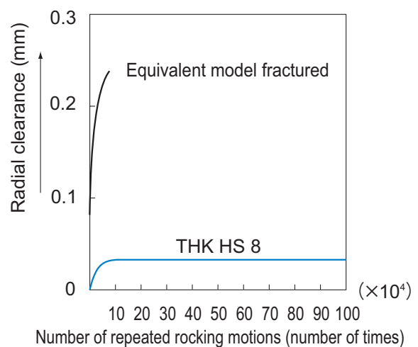
Fig.2 Wear Diagram
