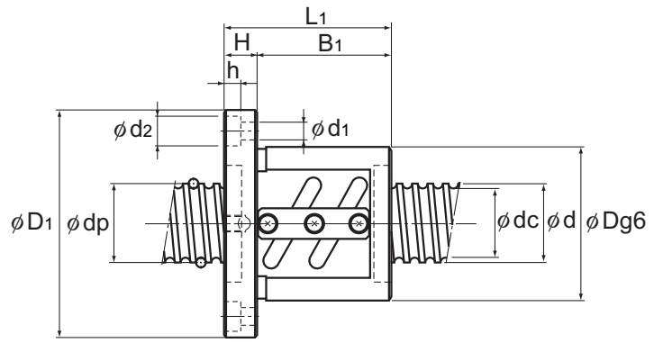
BIF
