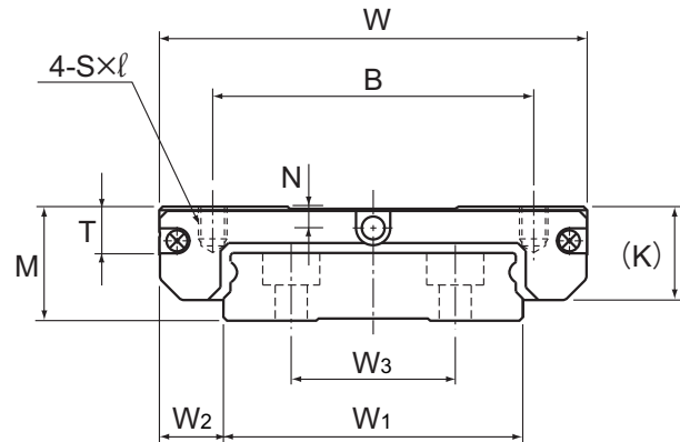
Model SRS15WM
