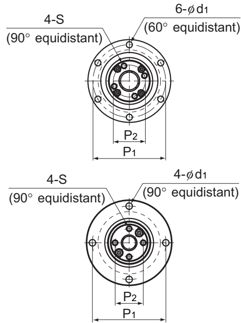
Models BNS 0812A and 1015A
