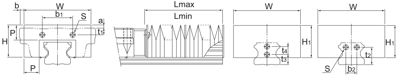
Models HSR15 to 30 Models HSR35 to 85
