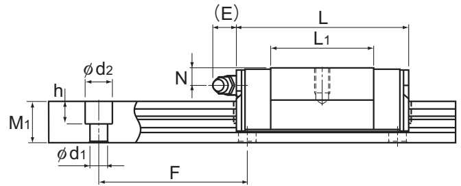
Model GSR25V-R
