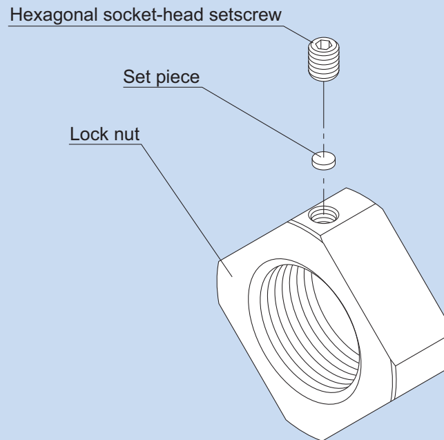
Fig.1 Structure of the Lock Nut
