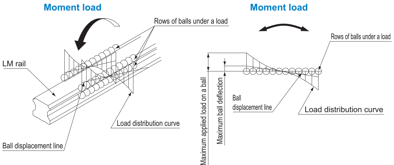
Fig.2 Ball Load when a Moment is Applied
