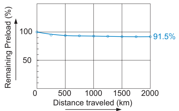
Fig.7 Distance Traveled and Remaining Preload
