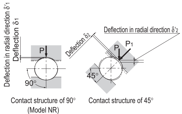
Fig.1 Deflection under a Radial Load
