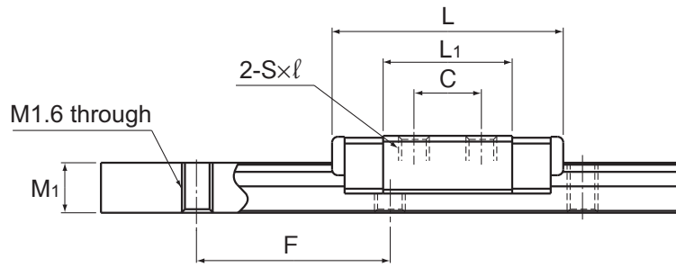
Model RSR3M
