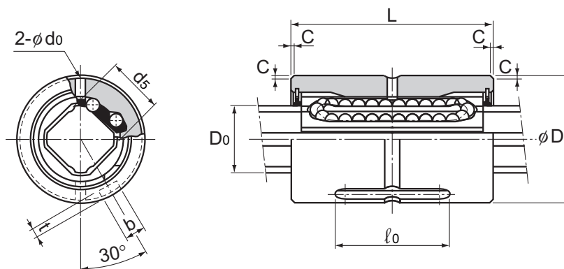
Model LBS10
