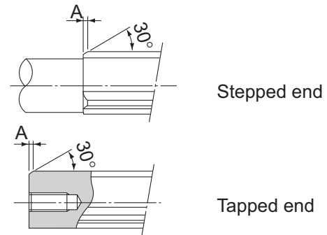
Fig.1 Chamfer A
