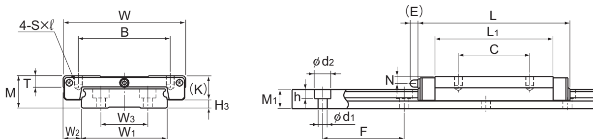
Models RSR14WV and 15WV/WVM/WN
