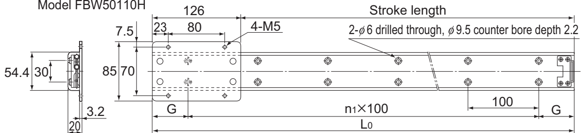
Model FBW50110H
