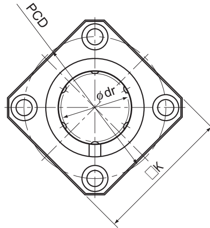
Model LMK
