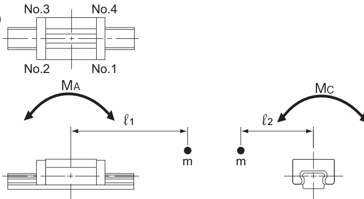
Fig.6 When One LM Block is Used
