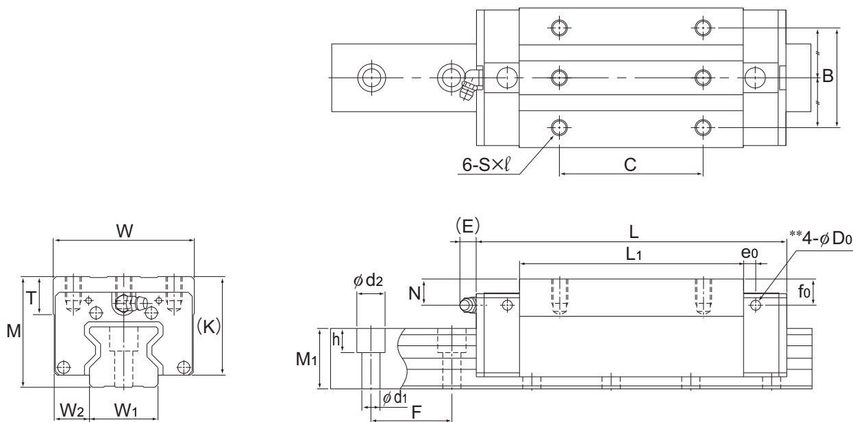
Models SRG25 to 65R/LR/LV
