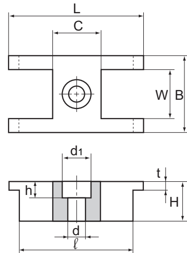
Model SMB
