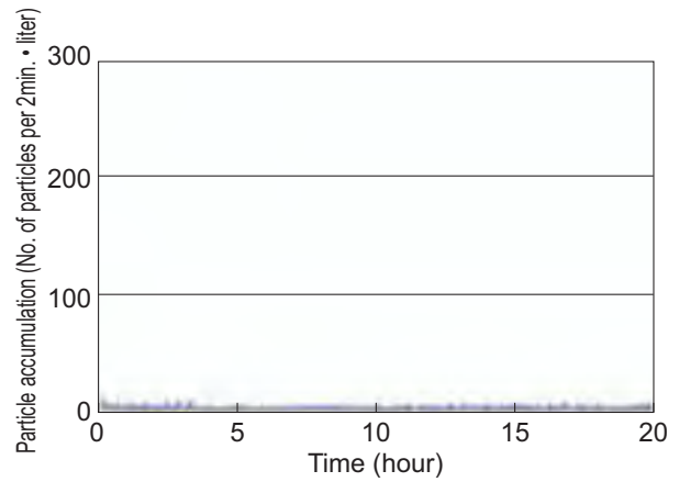
Caged Ball LM Guide Model SSR20
