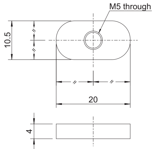
Fig.7 Plate Nut
