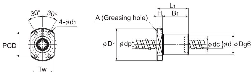
Models BTK 1006 and 1208
