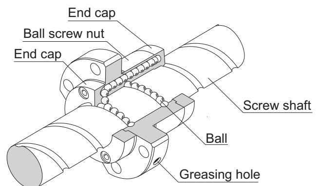
Example of Structure of Large lead Nut
