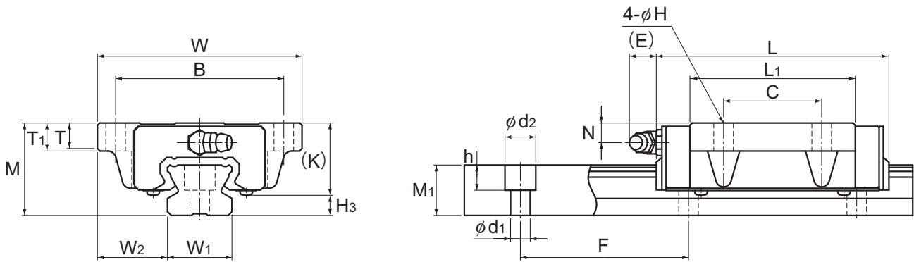
Model SR-M1TB
