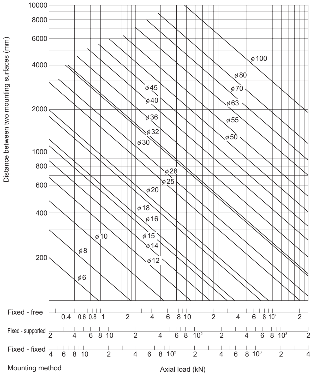
Fig.8 Permissible Tensile Compressive Load Diagram
