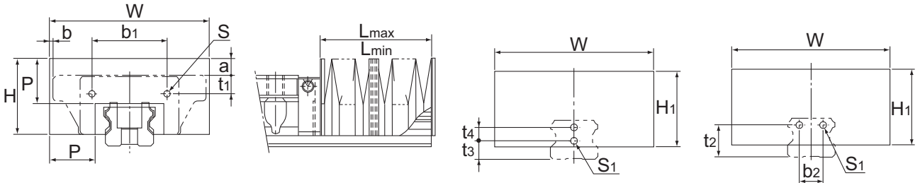
Models SHS15 to 30
