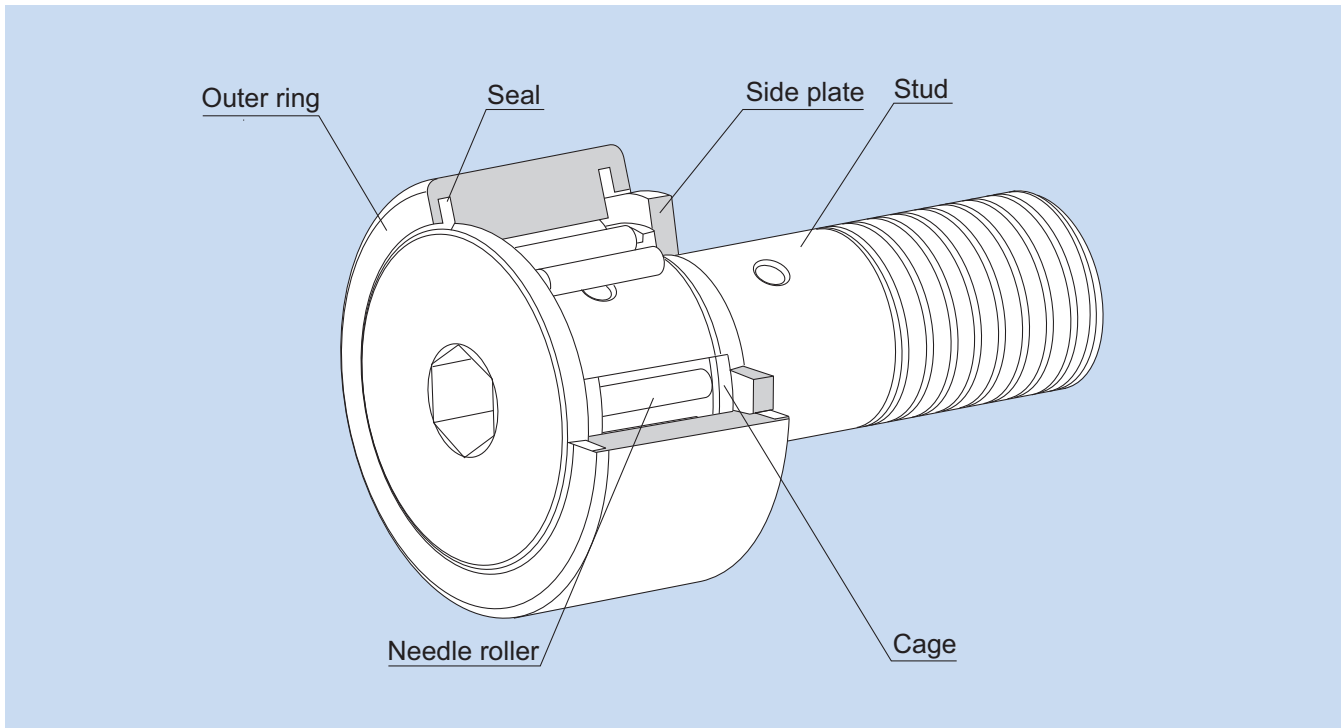
Fig.1 Structure of Cam Follower Model CF...UU-A
