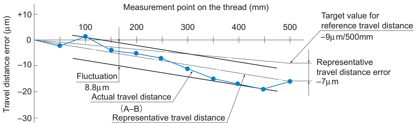
Fig.2 Measurement Data on Travel Distance Error
