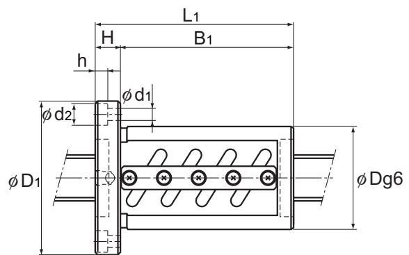
Model BIF
