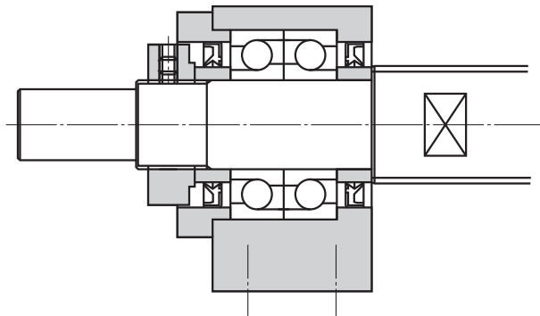
Model BK
