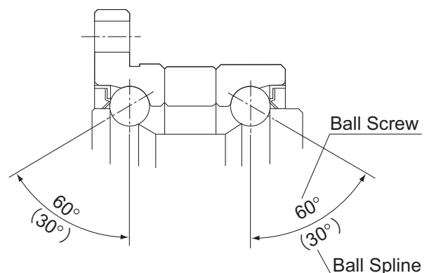
Fig.2 Structure of Support Bearing Model BNS
