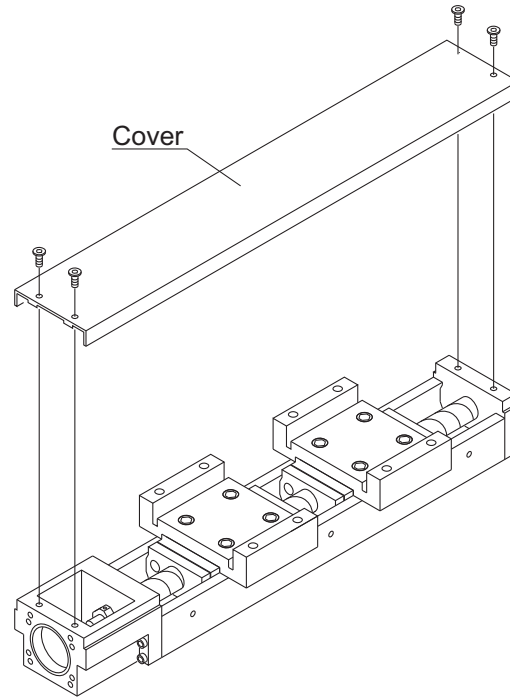
Model SKR33(with a Cover)
