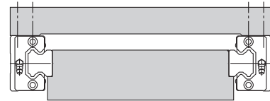
Fig.2 Mounting Structure for Model HSR-YR
