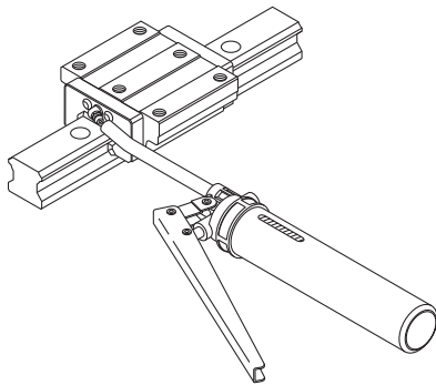
Fig.1 Lubrication Using a Grease Gun
