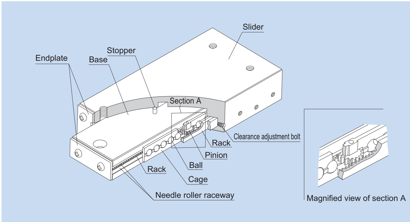
Fig.1 Structure of Linear Ball Slide Model LSP
