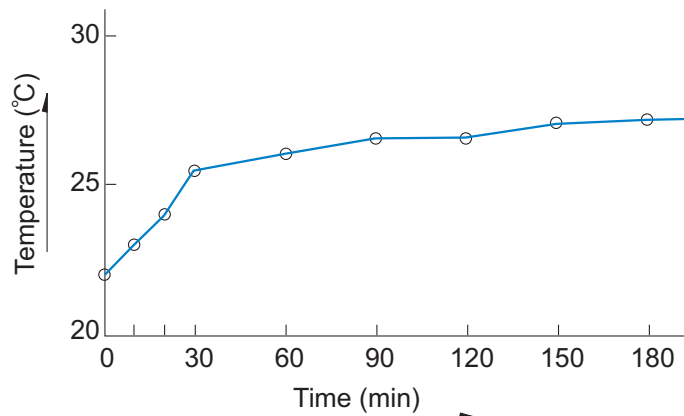
Fig.9 Ball Screw Heat Generation Data
