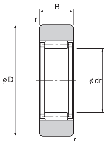
Model RNAS
