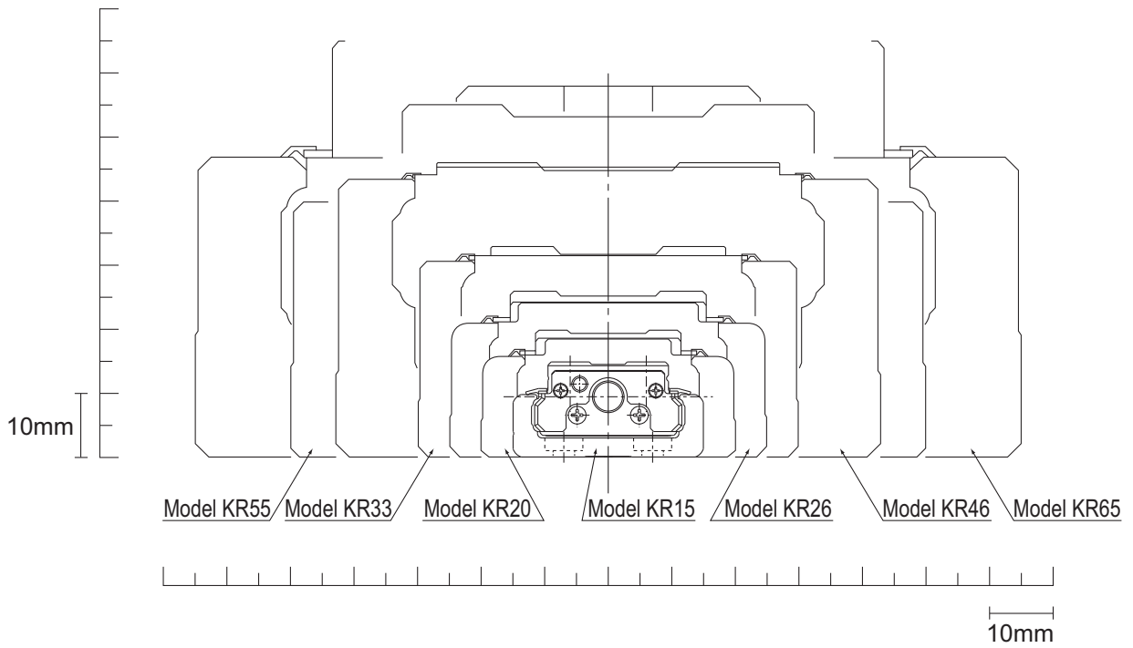
Fig.5 Cross Sectional Drawing
