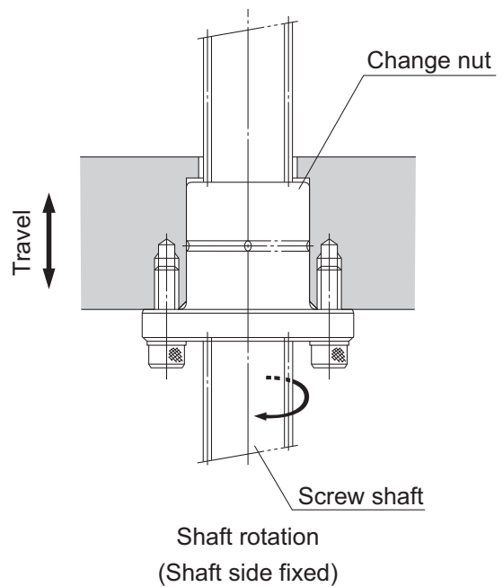
Fig.2 Recommended Mounting Orientation
