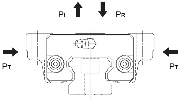
Fig.3 Model HSR
