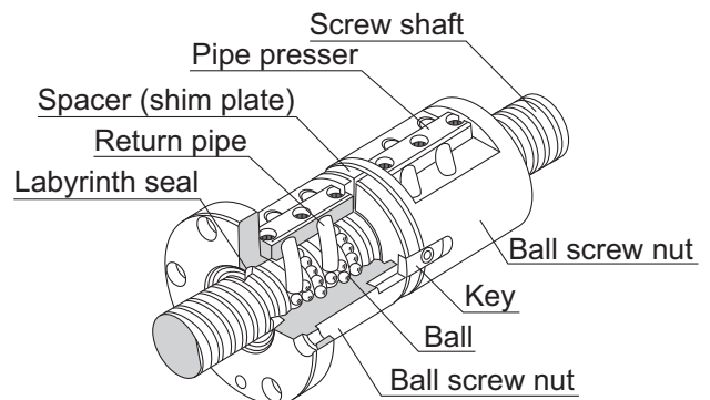
Example of Structure of Return-Pipe Nut
