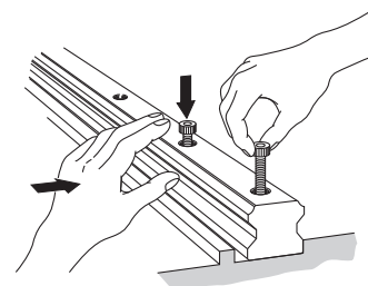
Fig.4 Checking with the Bolt for an Allowance
