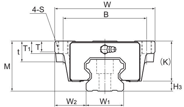
Models HSR45 to 85A/LA
