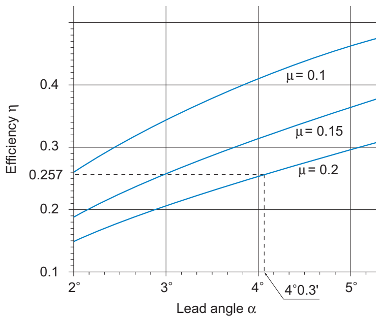
Fig.4 Efficiency
