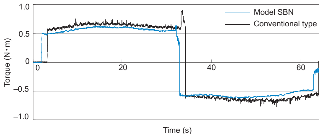
Fig.3 Torque Fluctuation Data
