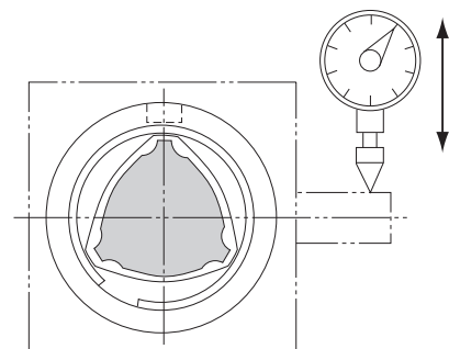
Fig.7 Measurement of Clearance in the Rotational Direction
