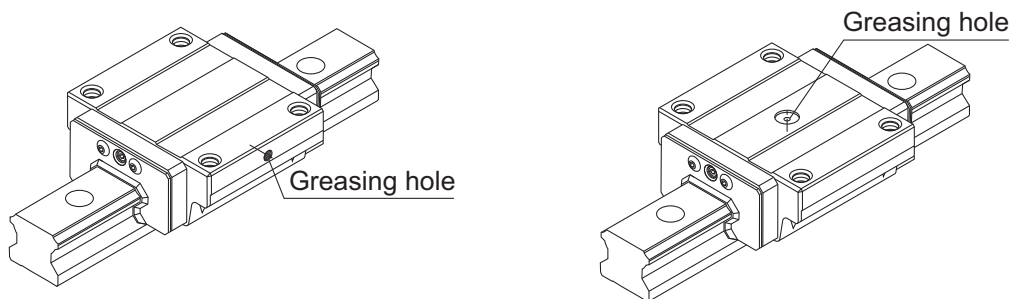
Type with a Greasing Hole Drilled on the Side Surface
