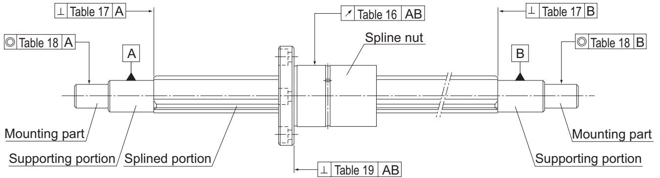
Fig.11 Accuracy Measurement Items of the Ball Spline
