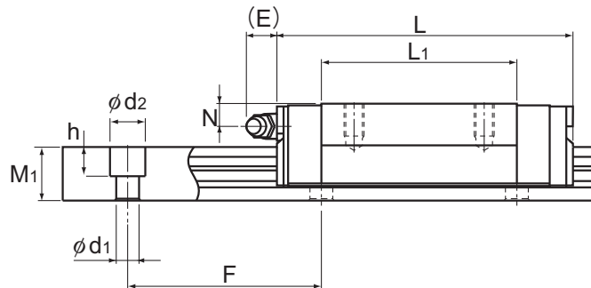
Model GSR-T-R
