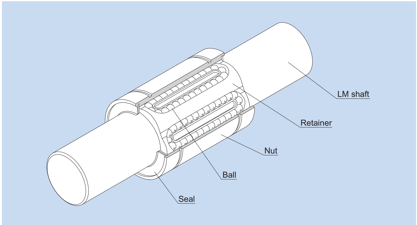
Fig.1 Structure of Linear Bushing Model LM···UU
