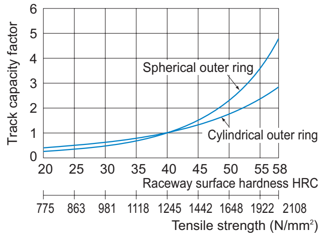
Fig.2 Track Capacity Factor
