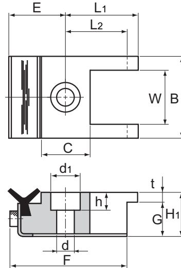
Model SEB
