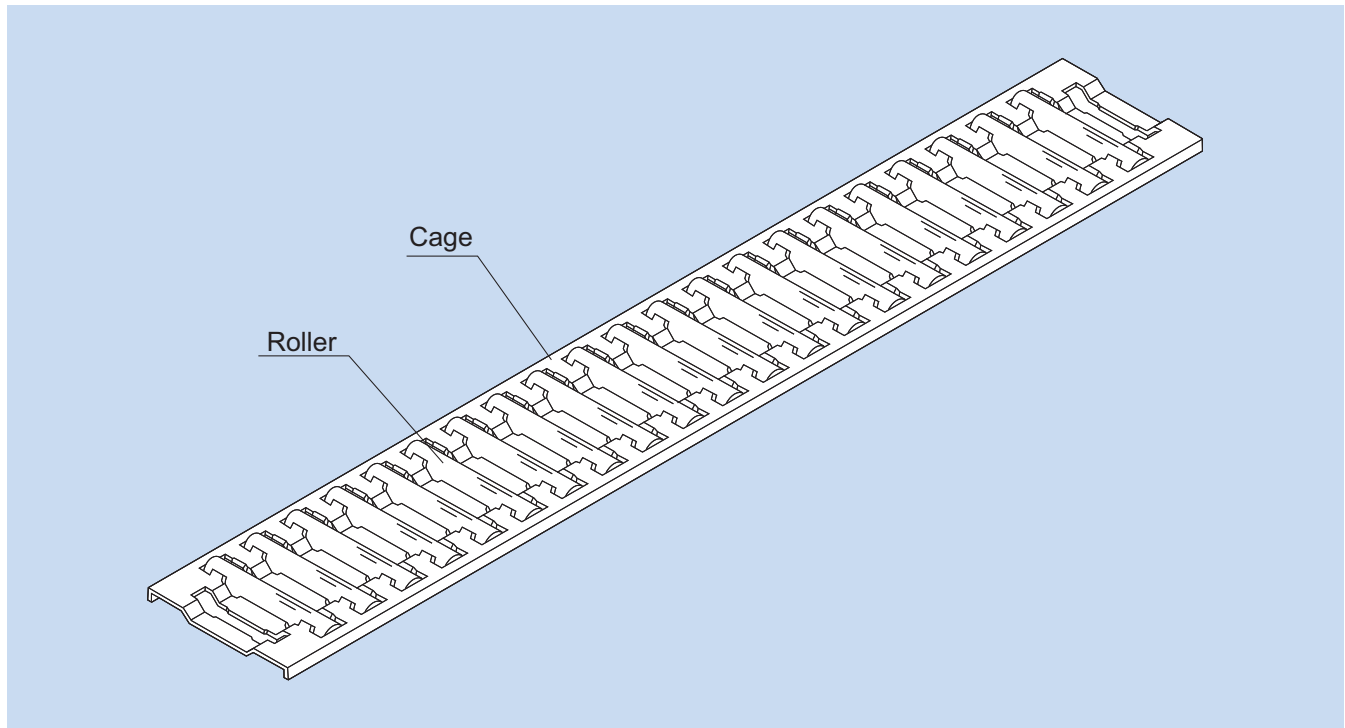
Fig.1 Structure of LM Flat Roller Model FT
