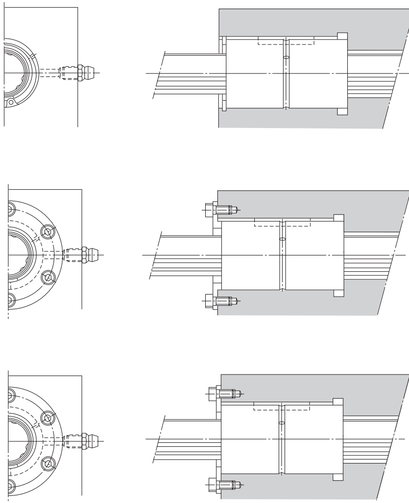
Fig.1 Examples of Fitting the Spline Nut
