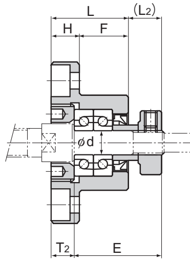
Mounting method B
