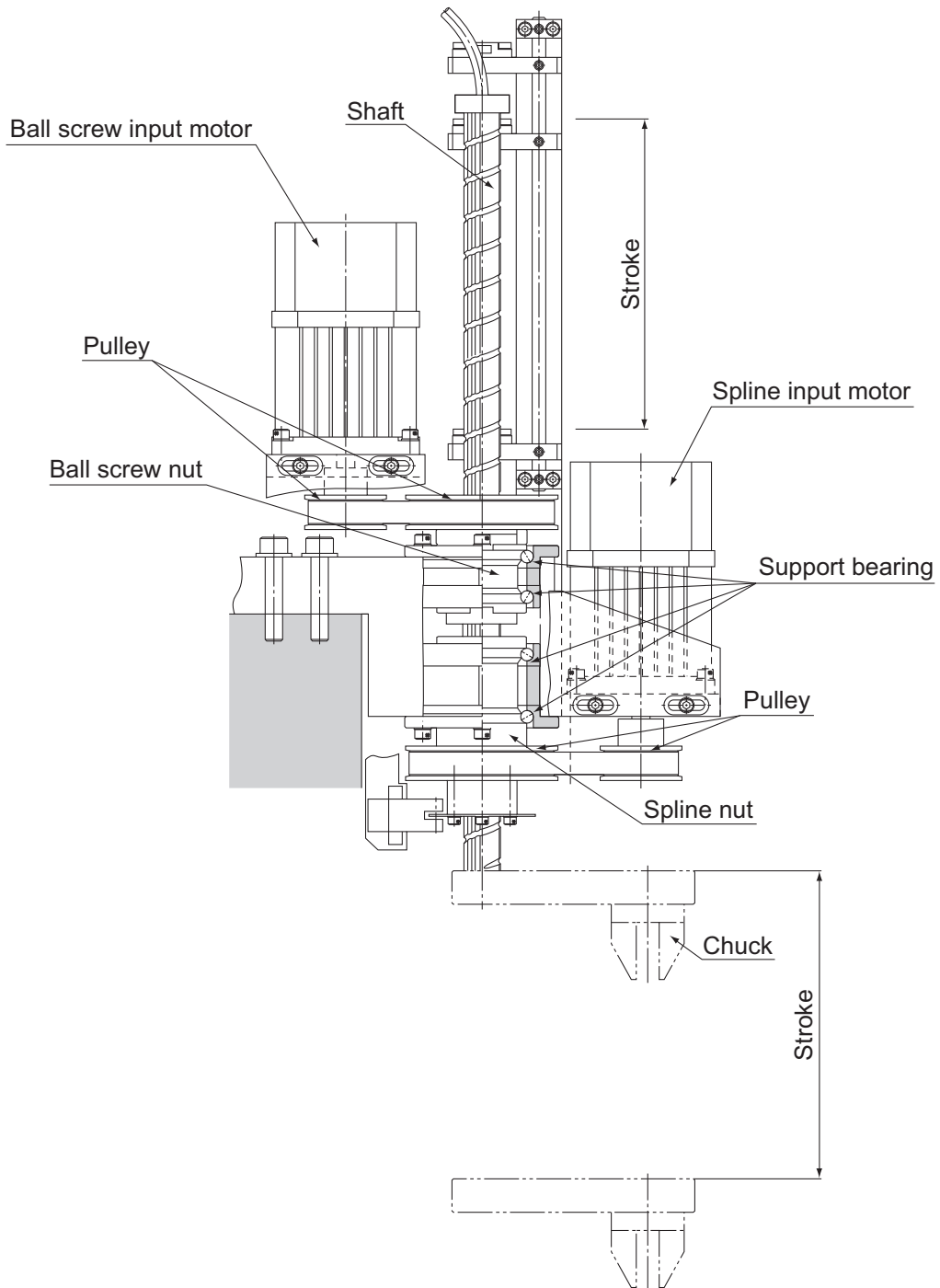
Fig.5 Example of Using Model BNS
