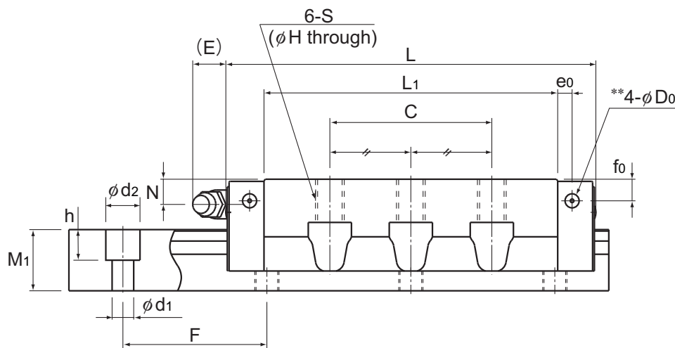
Model SNR-LC
