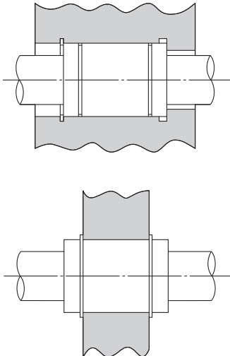
Fig.1 Snap Ring
