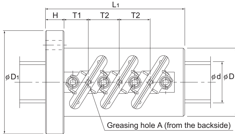
Models HBN4010 to 6320
