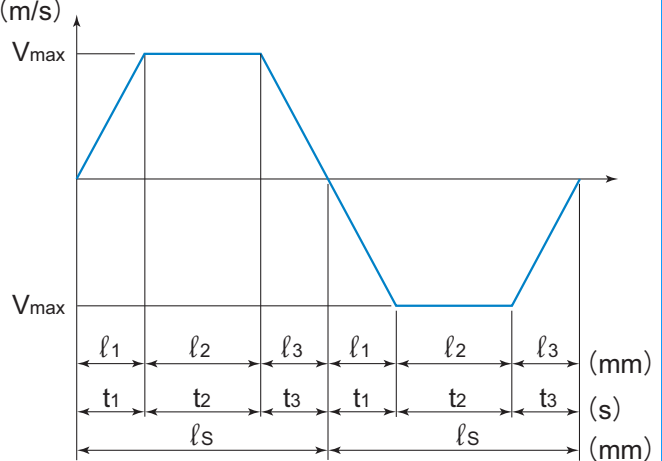
Velocity diagram
