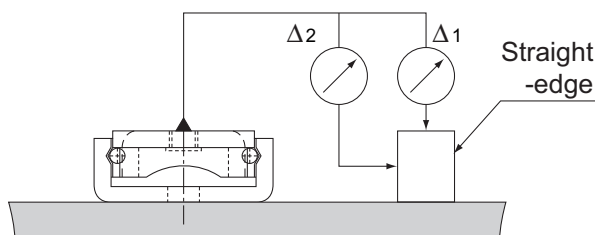
Fig.3 Method for Measuring Running Straightness
