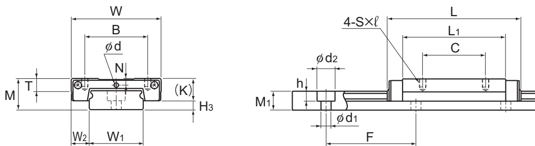
Models RSR9 and 12WV/WVM/WN
