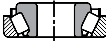
Type TSS Straight I.D., steep angle bearing; supports greater thrust but less radial load.
