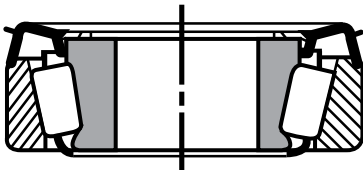
Type TSL Standard straight I.D. bearing; supports equal radial and thrust loads; sealed bearing.
