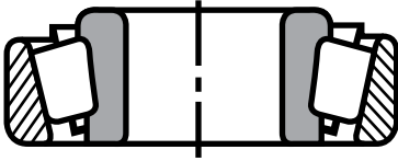
Type TS Standard straight I.D. bearing; supports equal radial and thrust loads.
