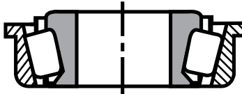
Type TSF Straight I.D. with flanged cup.
