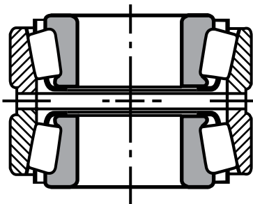
Type TDO Double cup, two single cones. Cones may be adjusted on instal- lation, or may be factory adjusted.
