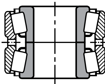
Type TNA Double cup, two single cones; front face of cones ground to a predetermined tolerance at the factory.
