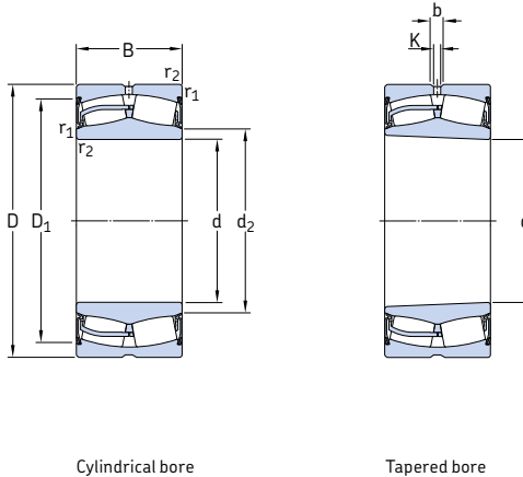
Cylindrical bore
