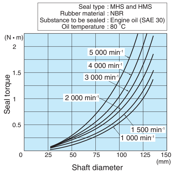
Fig. 1.6.9 Relation between shaft diameter and seal torque
