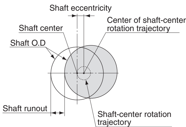
Fig. 1.5.5 Shaft runout
