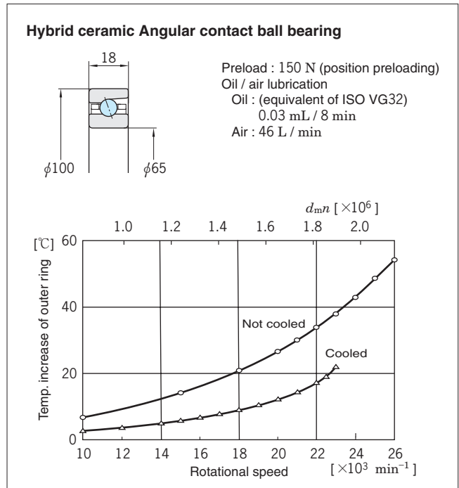
Fig. 11. 4 High speed performance with oil / air lub.
