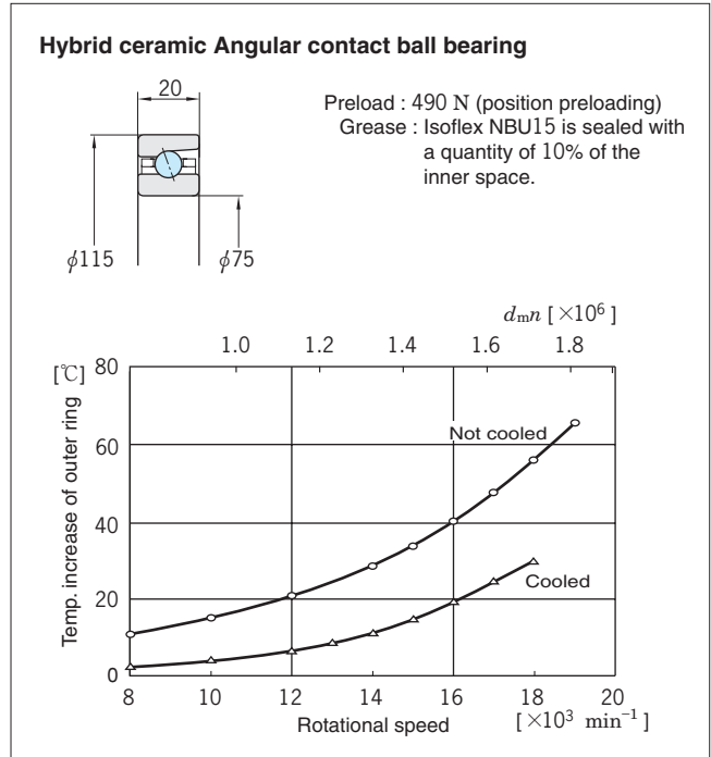
Fig. 11. 3 High speed performance with grease lub.
