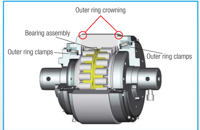
Typical installation of suitable bearing on jig Type 2
