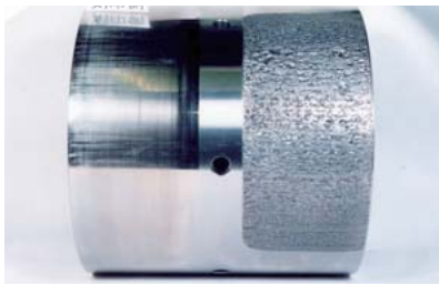
Raceway flaking
