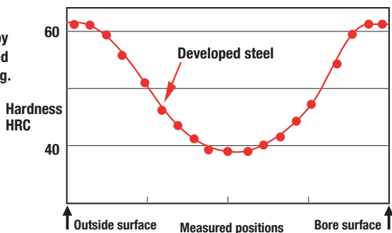
Typical hardness distribution of cored hardening outer ring
