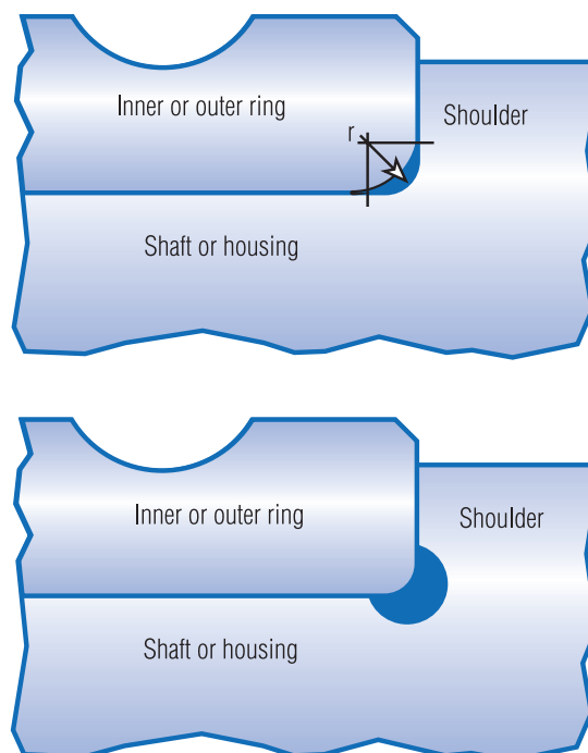
Fig. 21. Two methods of providing clearance for bearing corner.
