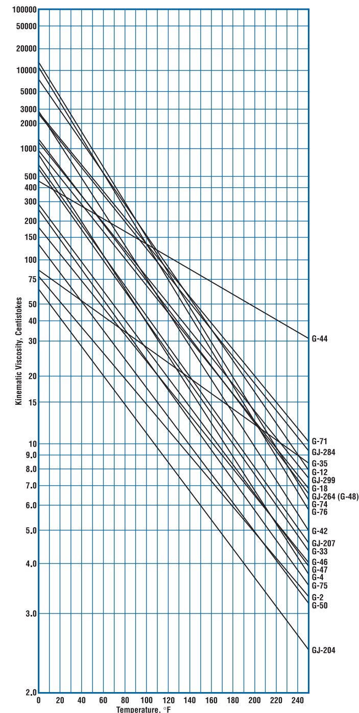
Viscosity graph for several typical grease lubricants.
