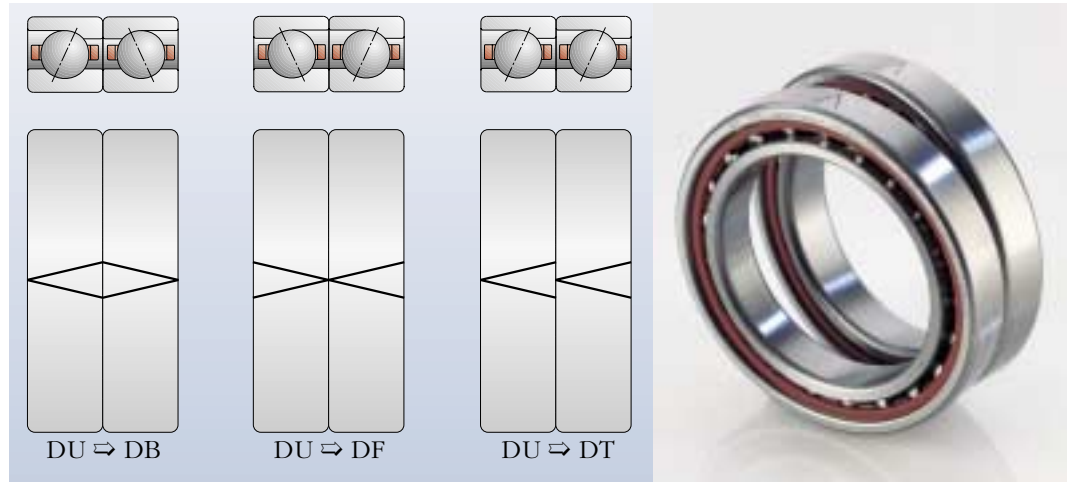
Fig. 1. Installation possibilities of a DU set
