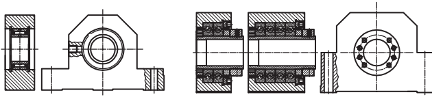
BLPB..N...2RS
