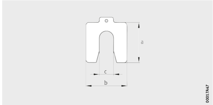
Figure 9 Shim, dimensions
